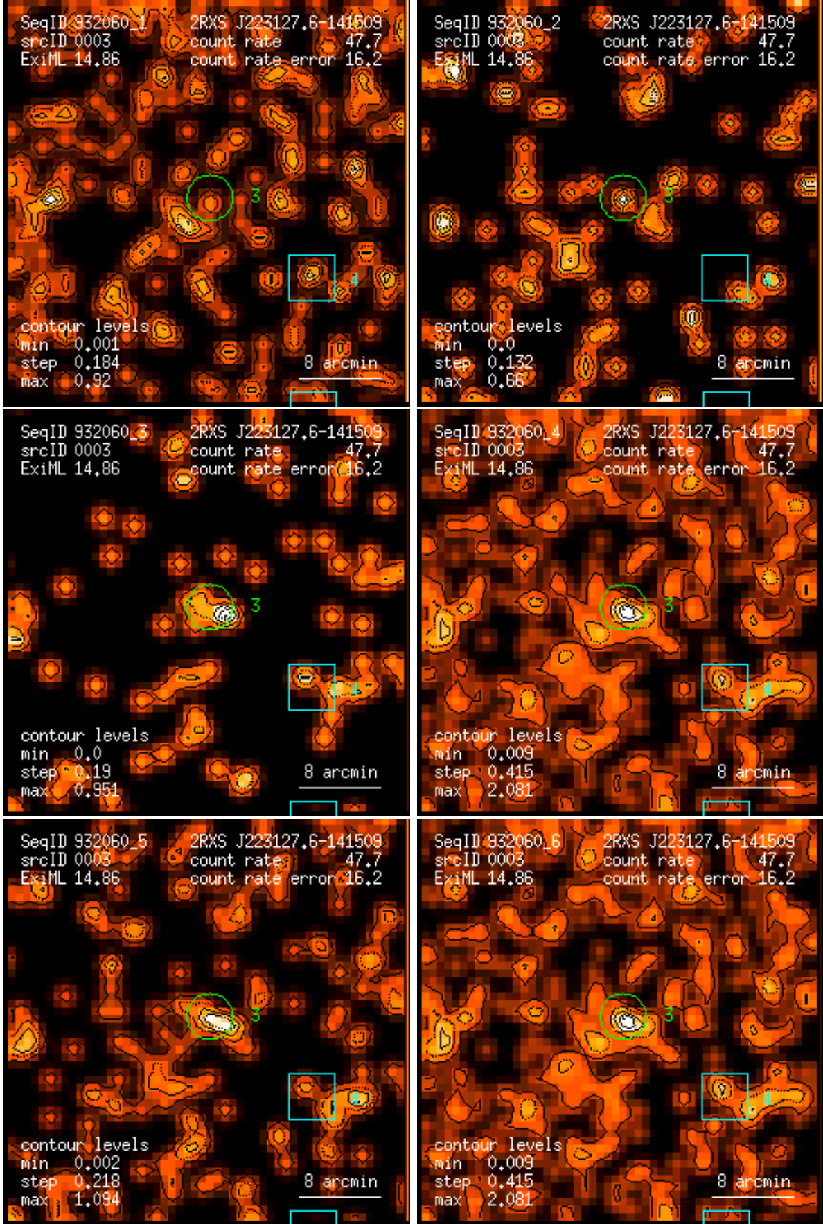
Figure 3: RASS 932060: detection 0003: band rate images, Gaussian filter: (1) PSPC channels 11 – 41, (2) 52 – 90, (3) 91 – 201, (4) 11 – 235, (5) 52 – 201, (6) 11 – 201. Broad band rates in counts/ks. Band rate contour levels in counts/ks/arcmin 2 .
