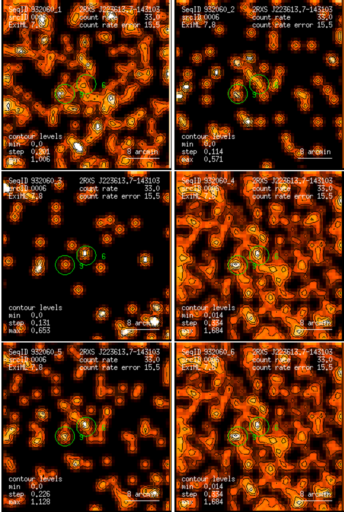
Figure 6: RASS 932060: detection 0006: band rate images, Gaussian filter: (1) PSPC channels 11 – 41, (2) 52 – 90, (3) 91 – 201, (4) 11 – 235, (5) 52 – 201, (6) 11 – 201. Broad band rates in counts/ks. Band rate contour levels in counts/ks/arcmin 2 .
