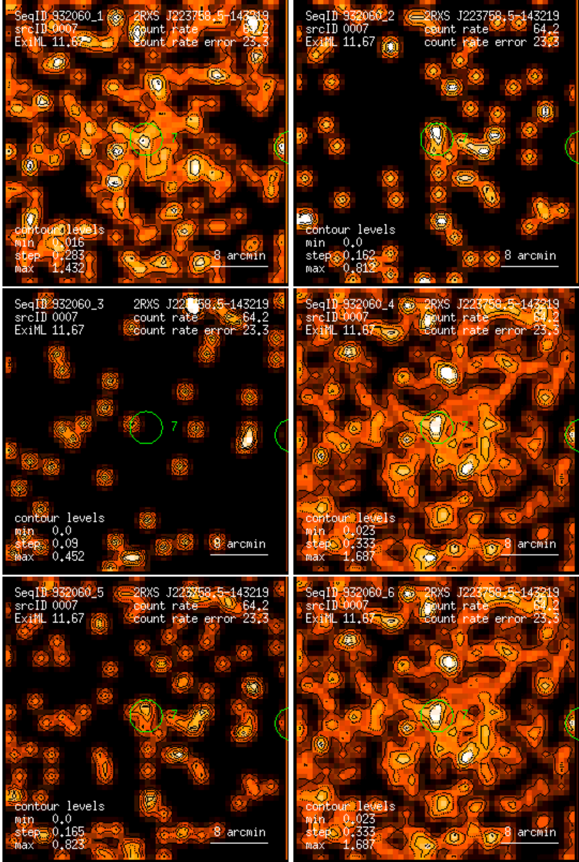
Figure 7: RASS 932060: detection 0007: band rate images, Gaussian filter: (1) PSPC channels 11 – 41, (2) 52 – 90, (3) 91 – 201, (4) 11 – 235, (5) 52 – 201, (6) 11 – 201. Broad band rates in counts/ks. Band rate contour levels in counts/ks/arcmin 2 .
