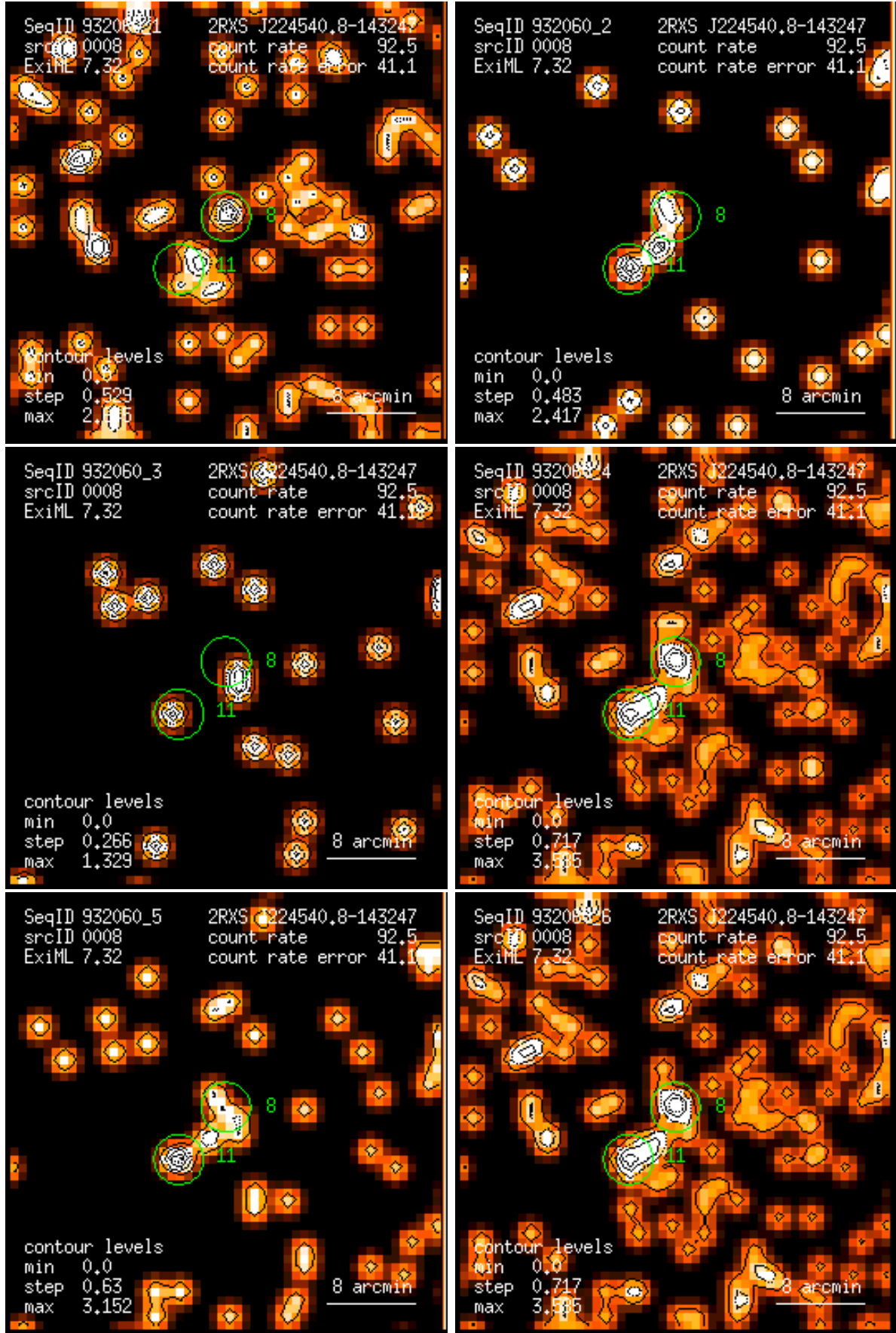
Figure 8: RASS 932060: detection 0008: band rate images, Gaussian filter: (1) PSPC channels 11 – 41, (2) 52 – 90, (3) 91 – 201, (4) 11 – 235, (5) 52 – 201, (6) 11 – 201. Broad band rates in counts/ks. Band rate contour levels in counts/ks/arcmin 2 .
