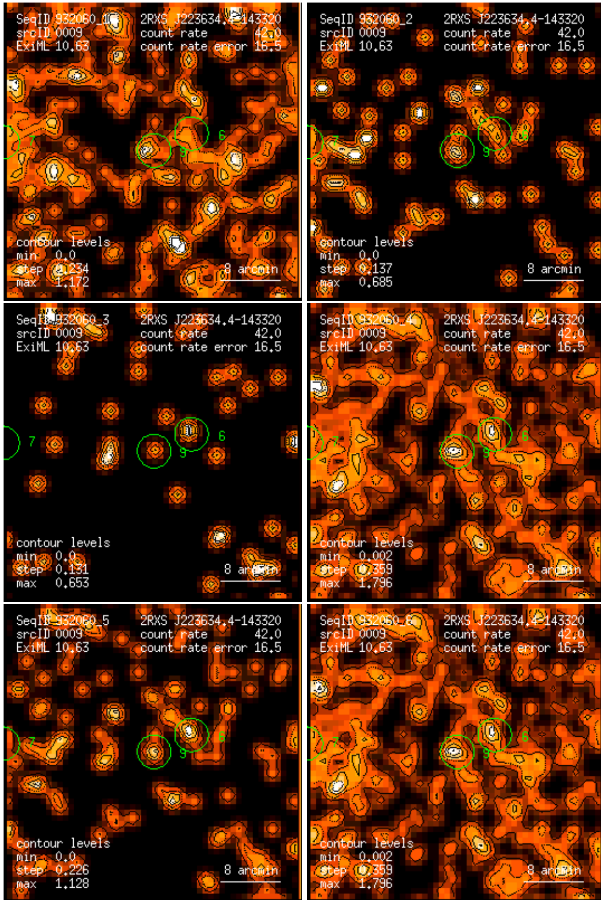
Figure 9: RASS 932060: detection 0009: band rate images, Gaussian filter: (1) PSPC channels 11 – 41, (2) 52 – 90, (3) 91 – 201, (4) 11 – 235, (5) 52 – 201, (6) 11 – 201. Broad band rates in counts/ks. Band rate contour levels in counts/ks/arcmin 2 .
