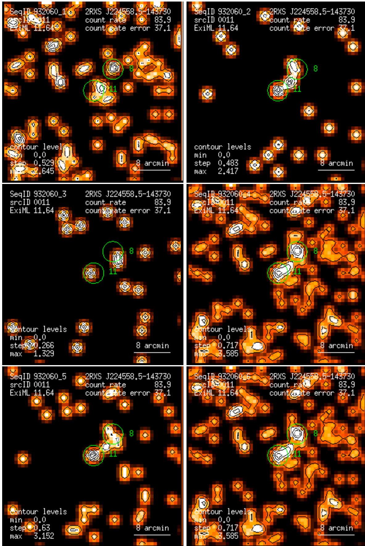
Figure 11: RASS 932060: detection 0011: band rate images, Gaussian filter: (1) PSPC channels 11 – 41, (2) 52 – 90, (3) 91 – 201, (4) 11 – 235, (5) 52 – 201, (6) 11 – 201. Broad band rates in counts/ks. Band rate contour levels in counts/ks/arcmin 2 .
