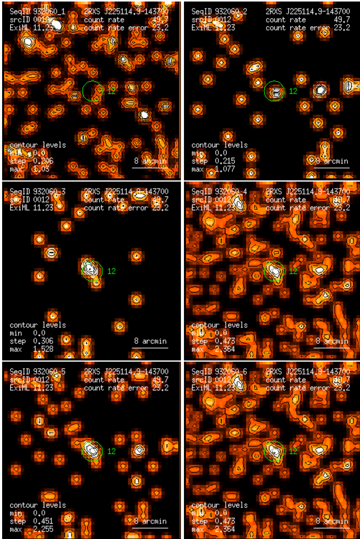
Figure 12: RASS 932060: detection 0012: band rate images, Gaussian filter: (1) PSPC channels 11 – 41, (2) 52 – 90, (3) 91 – 201, (4) 11 – 235, (5) 52 – 201, (6) 11 – 201. Broad band rates in counts/ks. Band rate contour levels in counts/ks/arcmin 2 .
