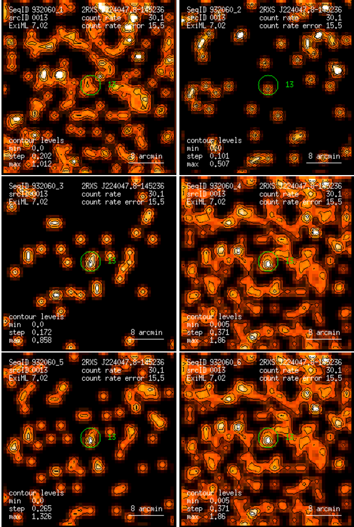
Figure 13: RASS 932060: detection 0013: band rate images, Gaussian filter: (1) PSPC channels 11 – 41, (2) 52 – 90, (3) 91 – 201, (4) 11 – 235, (5) 52 – 201, (6) 11 – 201. Broad band rates in counts/ks. Band rate contour levels in counts/ks/arcmin 2 .
