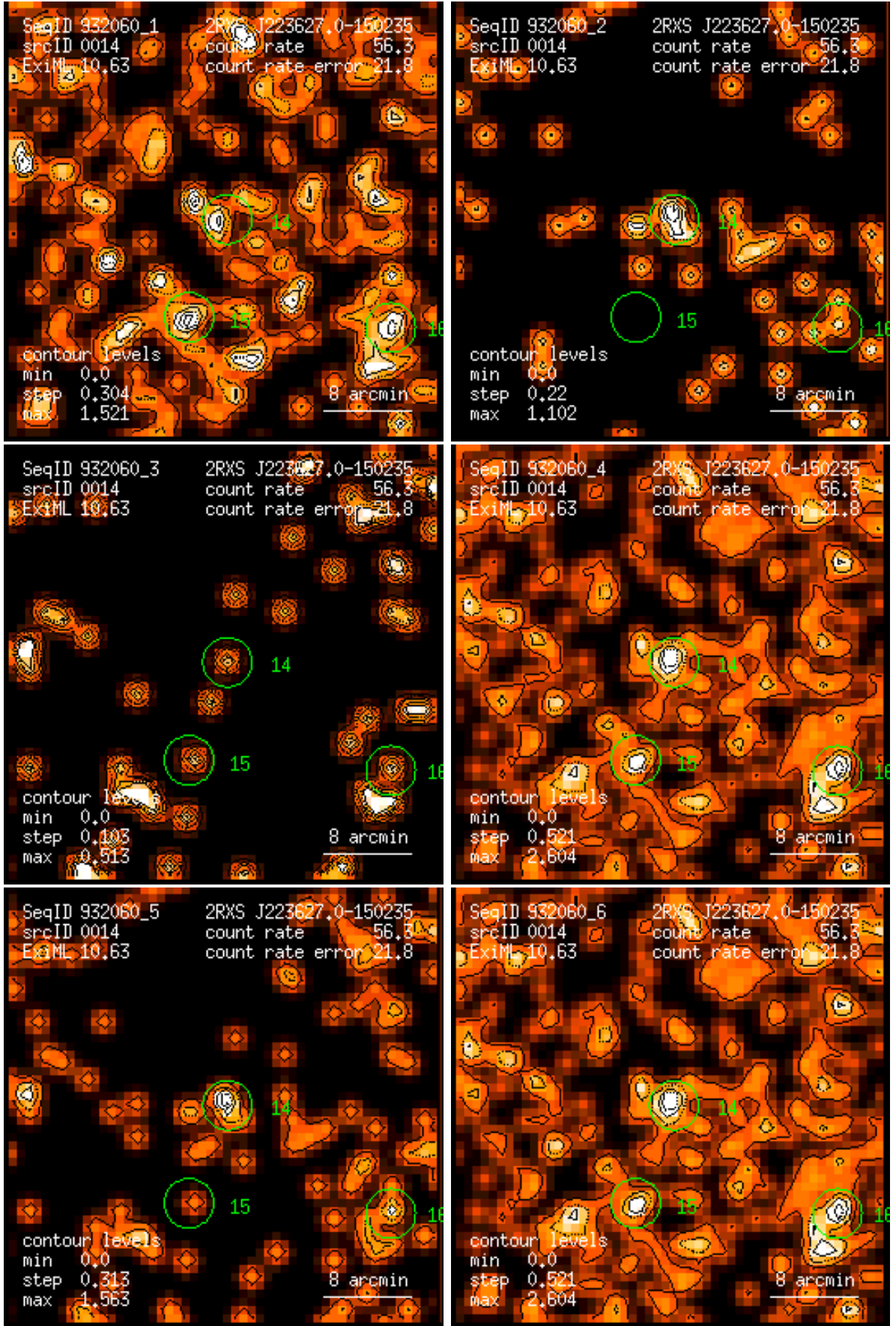
Figure 14: RASS 932060: detection 0014: band rate images, Gaussian filter: (1) PSPC channels 11 – 41, (2) 52 – 90, (3) 91 – 201, (4) 11 – 235, (5) 52 – 201, (6) 11 – 201. Broad band rates in counts/ks. Band rate contour levels in counts/ks/arcmin 2 .
