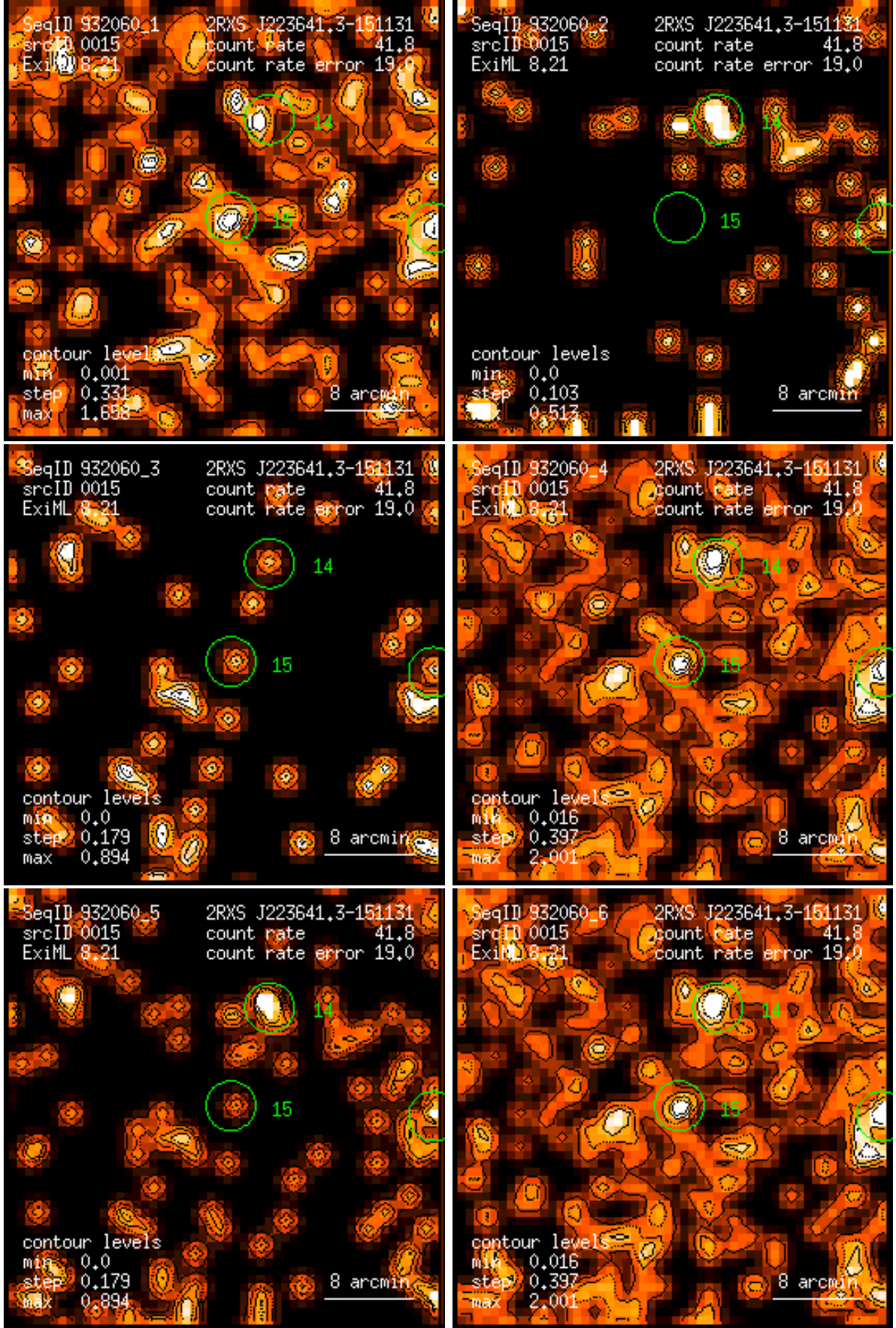
Figure 15: RASS 932060: detection 0015: band rate images, Gaussian filter: (1) PSPC channels 11 – 41, (2) 52 – 90, (3) 91 – 201, (4) 11 – 235, (5) 52 – 201, (6) 11 – 201. Broad band rates in counts/ks. Band rate contour levels in counts/ks/arcmin 2 .
