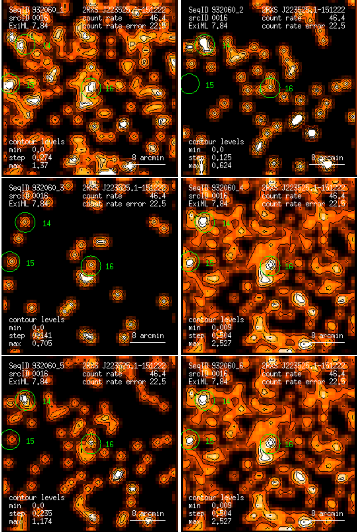
Figure 16: RASS 932060: detection 0016: band rate images, Gaussian filter: (1) PSPC channels 11 – 41, (2) 52 – 90, (3) 91 – 201, (4) 11 – 235, (5) 52 – 201, (6) 11 – 201. Broad band rates in counts/ks. Band rate contour levels in counts/ks/arcmin 2 .
