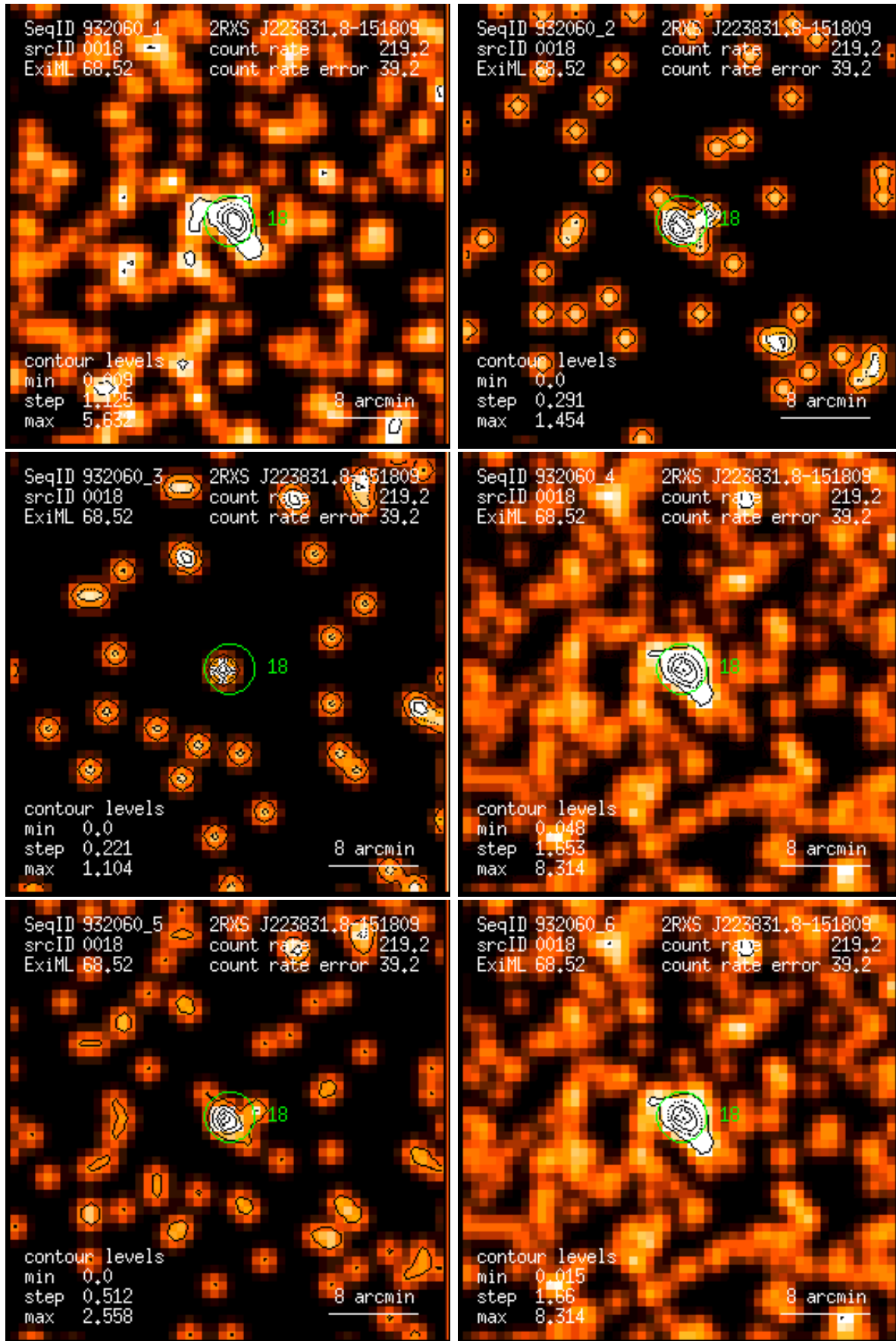
Figure 18: RASS 932060: detection 0018: band rate images, Gaussian filter: (1) PSPC channels 11 – 41, (2) 52 – 90, (3) 91 – 201, (4) 11 – 235, (5) 52 – 201, (6) 11 – 201. Broad band rates in counts/ks. Band rate contour levels in counts/ks/arcmin 2 .
