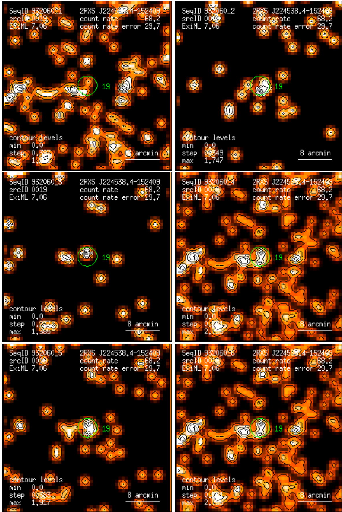
Figure 19: RASS 932060: detection 0019: band rate images, Gaussian filter: (1) PSPC channels 11 – 41, (2) 52 – 90, (3) 91 – 201, (4) 11 – 235, (5) 52 – 201, (6) 11 – 201. Broad band rates in counts/ks. Band rate contour levels in counts/ks/arcmin 2 .
