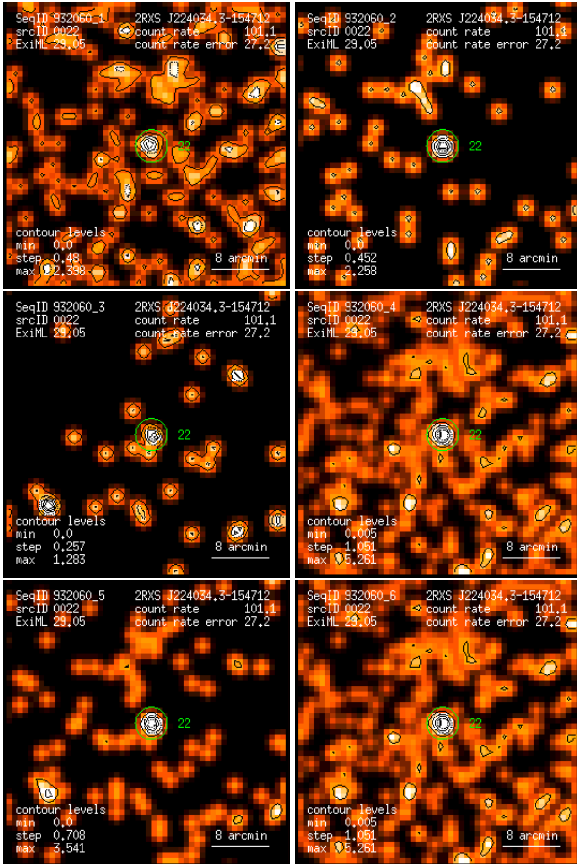
Figure 22: RASS 932060: detection 0022: band rate images, Gaussian filter: (1) PSPC channels 11 – 41, (2) 52 – 90, (3) 91 – 201, (4) 11 – 235, (5) 52 – 201, (6) 11 – 201. Broad band rates in counts/ks. Band rate contour levels in counts/ks/arcmin 2 .
