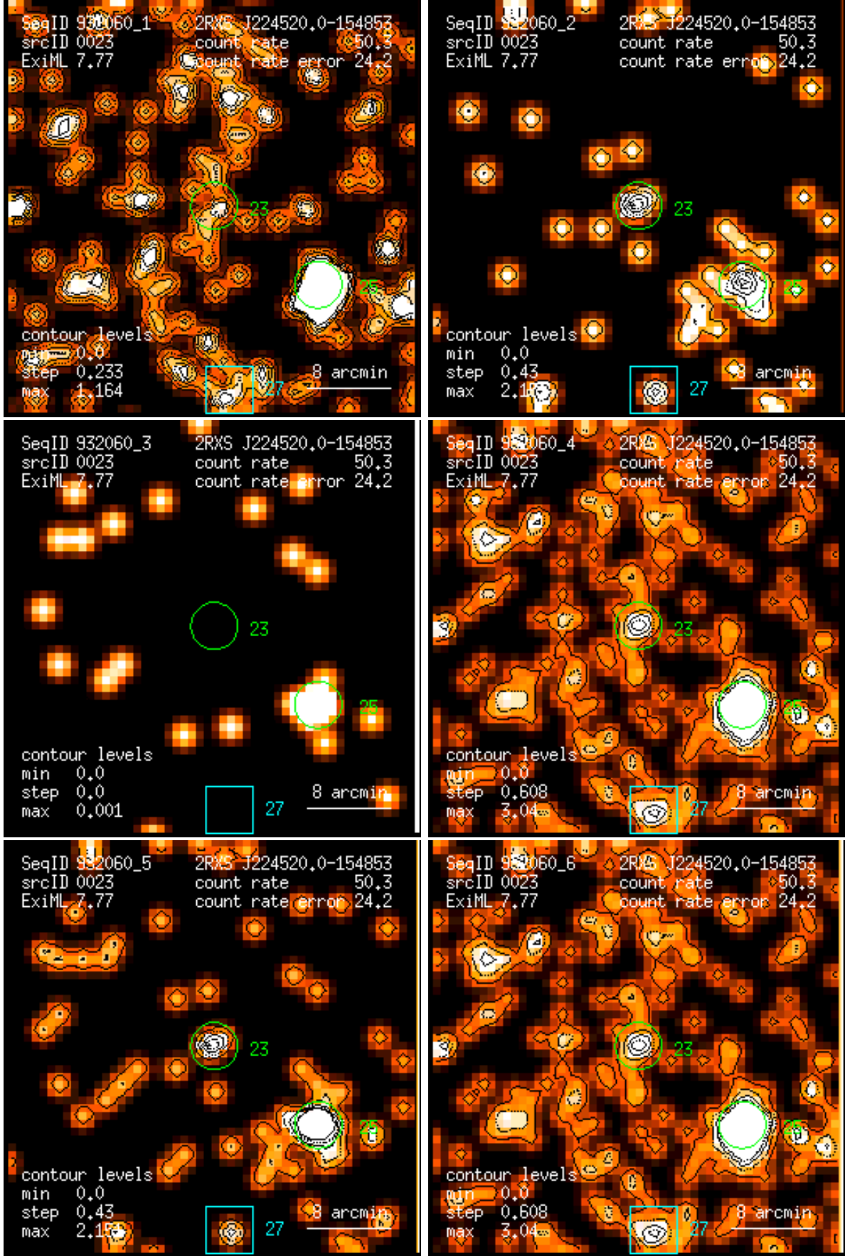
Figure 23: RASS 932060: detection 0023: band rate images, Gaussian filter: (1) PSPC channels 11 – 41, (2) 52 – 90, (3) 91 – 201, (4) 11 – 235, (5) 52 – 201, (6) 11 – 201. Broad band rates in counts/ks. Band rate contour levels in counts/ks/arcmin 2 .
