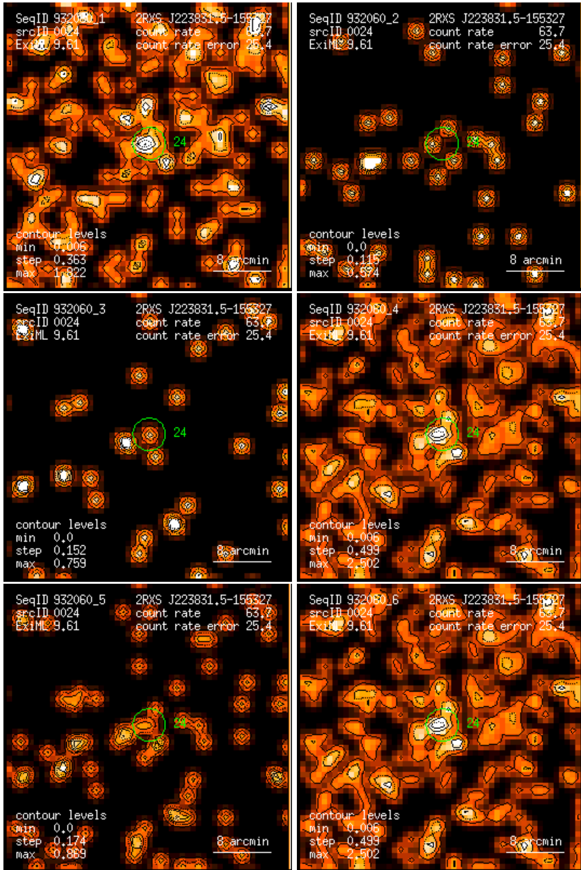
Figure 24: RASS 932060: detection 0024: band rate images, Gaussian filter: (1) PSPC channels 11 – 41, (2) 52 – 90, (3) 91 – 201, (4) 11 – 235, (5) 52 – 201, (6) 11 – 201. Broad band rates in counts/ks. Band rate contour levels in counts/ks/arcmin 2 .
