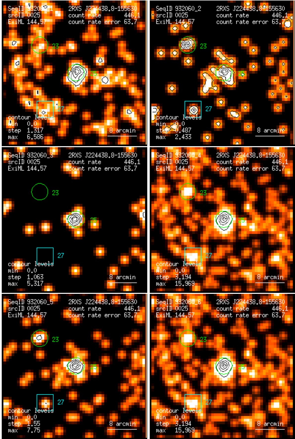
Figure 25: RASS 932060: detection 0025: band rate images, Gaussian filter: (1) PSPC channels 11 – 41, (2) 52 – 90, (3) 91 – 201, (4) 11 – 235, (5) 52 – 201, (6) 11 – 201. Broad band rates in counts/ks. Band rate contour levels in counts/ks/arcmin 2 .
