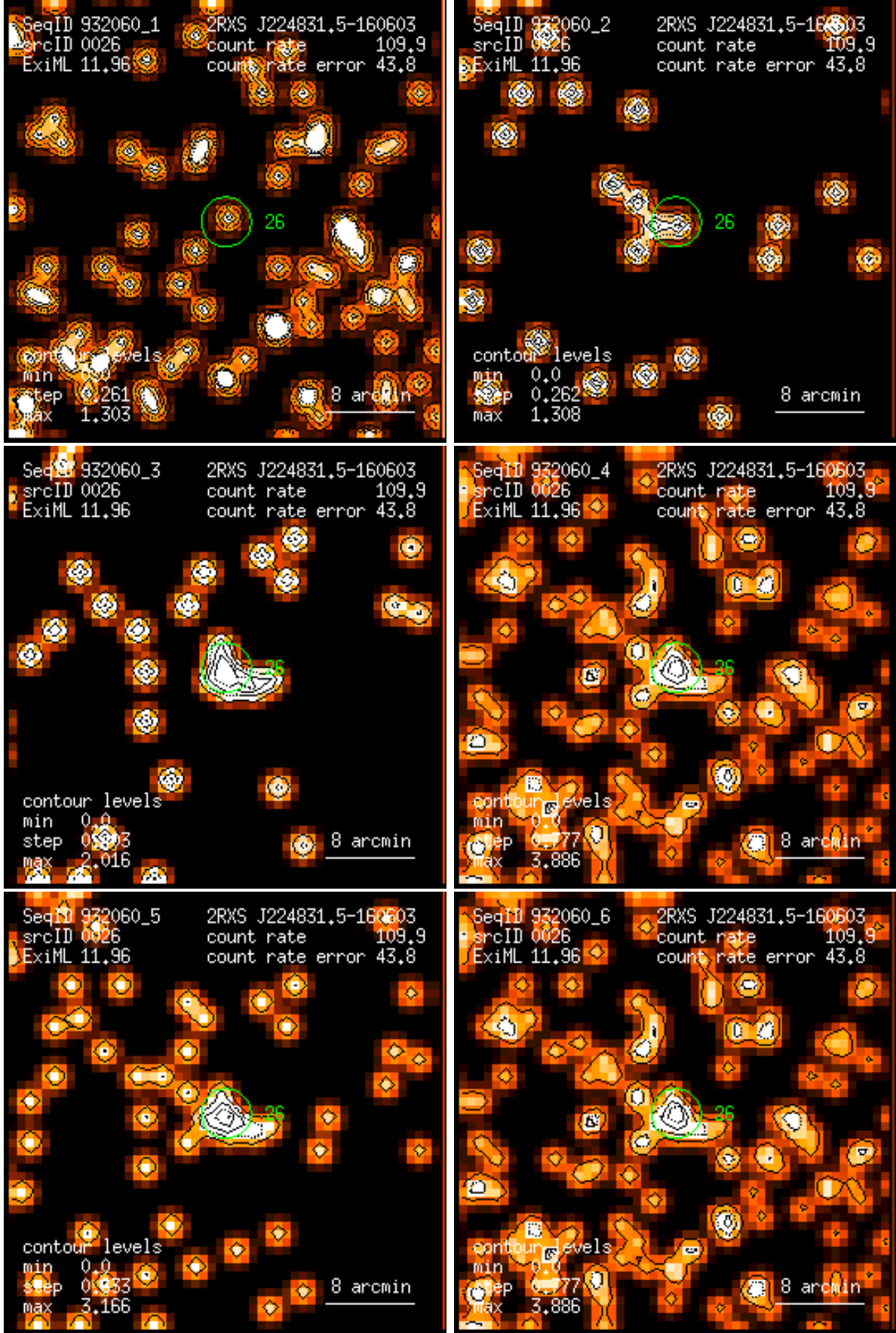
Figure 26: RASS 932060: detection 0026: band rate images, Gaussian filter: (1) PSPC channels 11 – 41, (2) 52 – 90, (3) 91 – 201, (4) 11 – 235, (5) 52 – 201, (6) 11 – 201. Broad band rates in counts/ks. Band rate contour levels in counts/ks/arcmin 2 .
