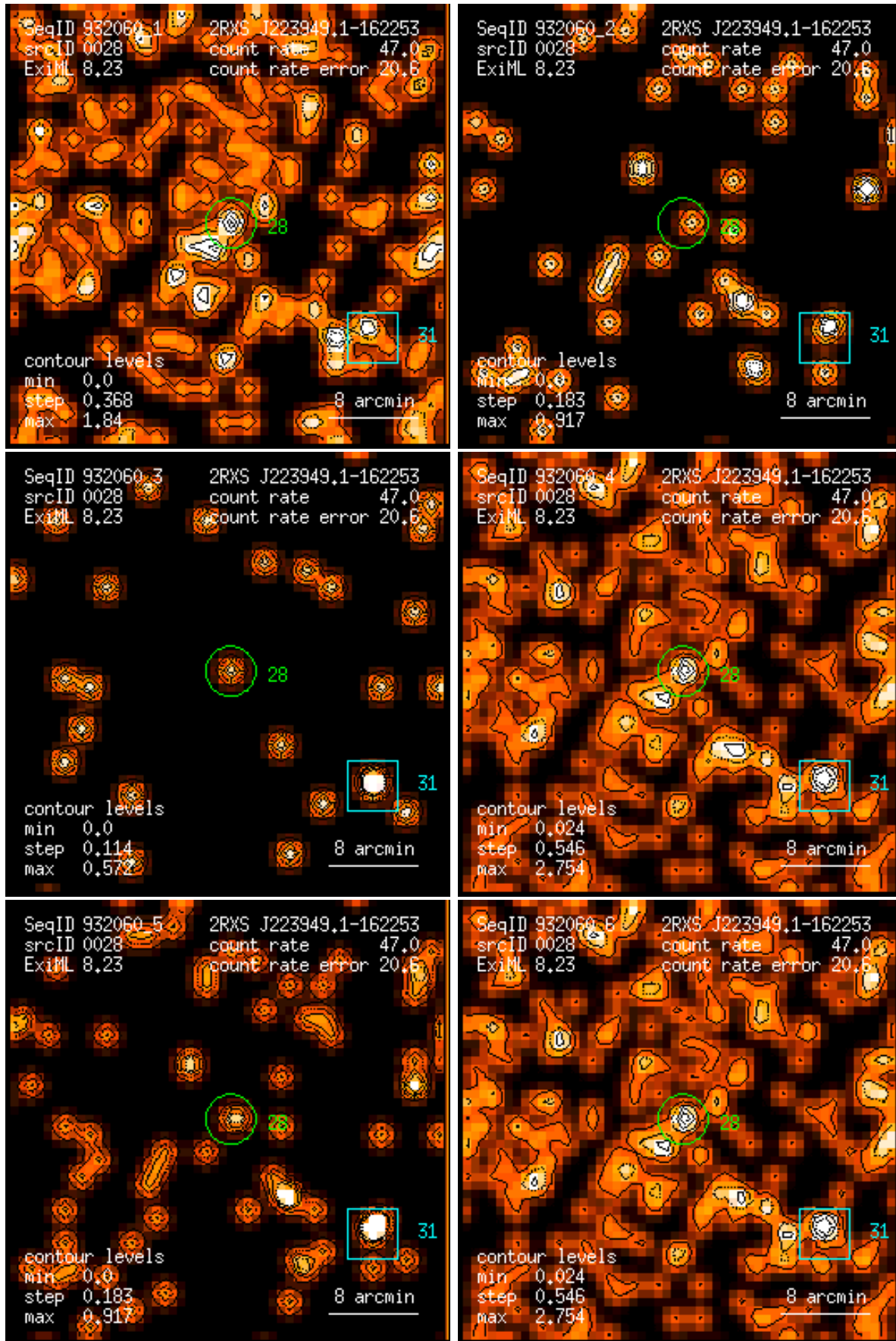
Figure 28: RASS 932060: detection 0028: band rate images, Gaussian filter: (1) PSPC channels 11 – 41, (2) 52 – 90, (3) 91 – 201, (4) 11 – 235, (5) 52 – 201, (6) 11 – 201. Broad band rates in counts/ks. Band rate contour levels in counts/ks/arcmin 2 .
