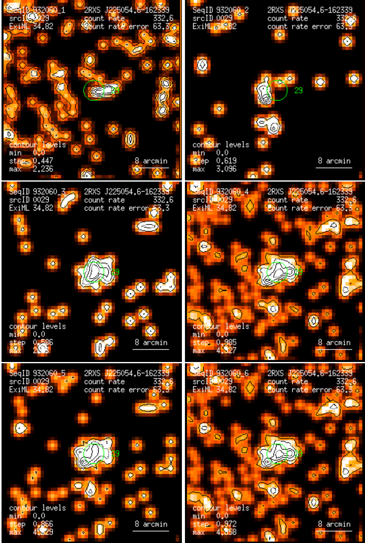
Figure 29: RASS 932060: detection 0029: band rate images, Gaussian filter: (1) PSPC channels 11 – 41, (2) 52 – 90, (3) 91 – 201, (4) 11 – 235, (5) 52 – 201, (6) 11 – 201. Broad band rates in counts/ks. Band rate contour levels in counts/ks/arcmin 2 .
