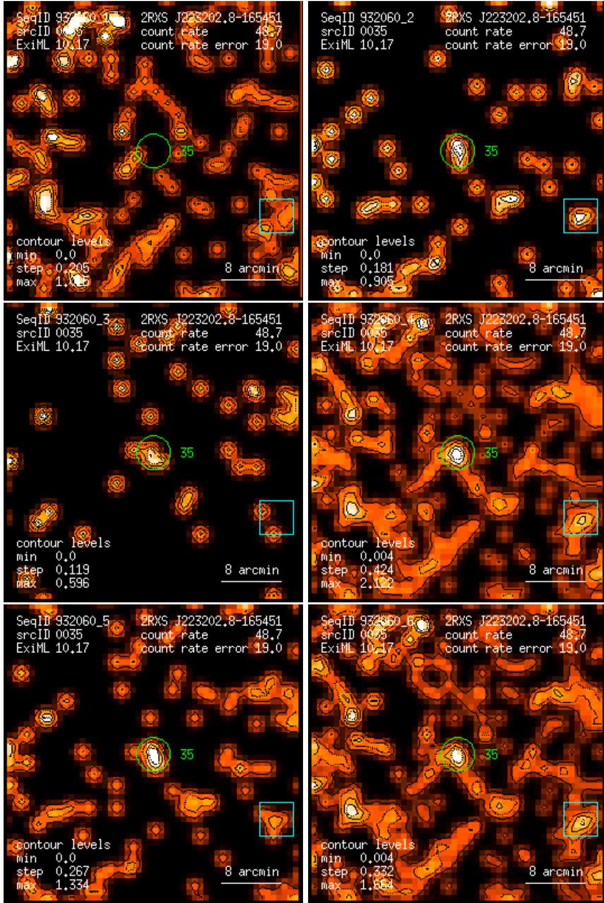
Figure 35: RASS 932060: detection 0035: band rate images, Gaussian filter: (1) PSPC channels 11 – 41, (2) 52 – 90, (3) 91 – 201, (4) 11 – 235, (5) 52 – 201, (6) 11 – 201. Broad band rates in counts/ks. Band rate contour levels in counts/ks/arcmin 2 .
