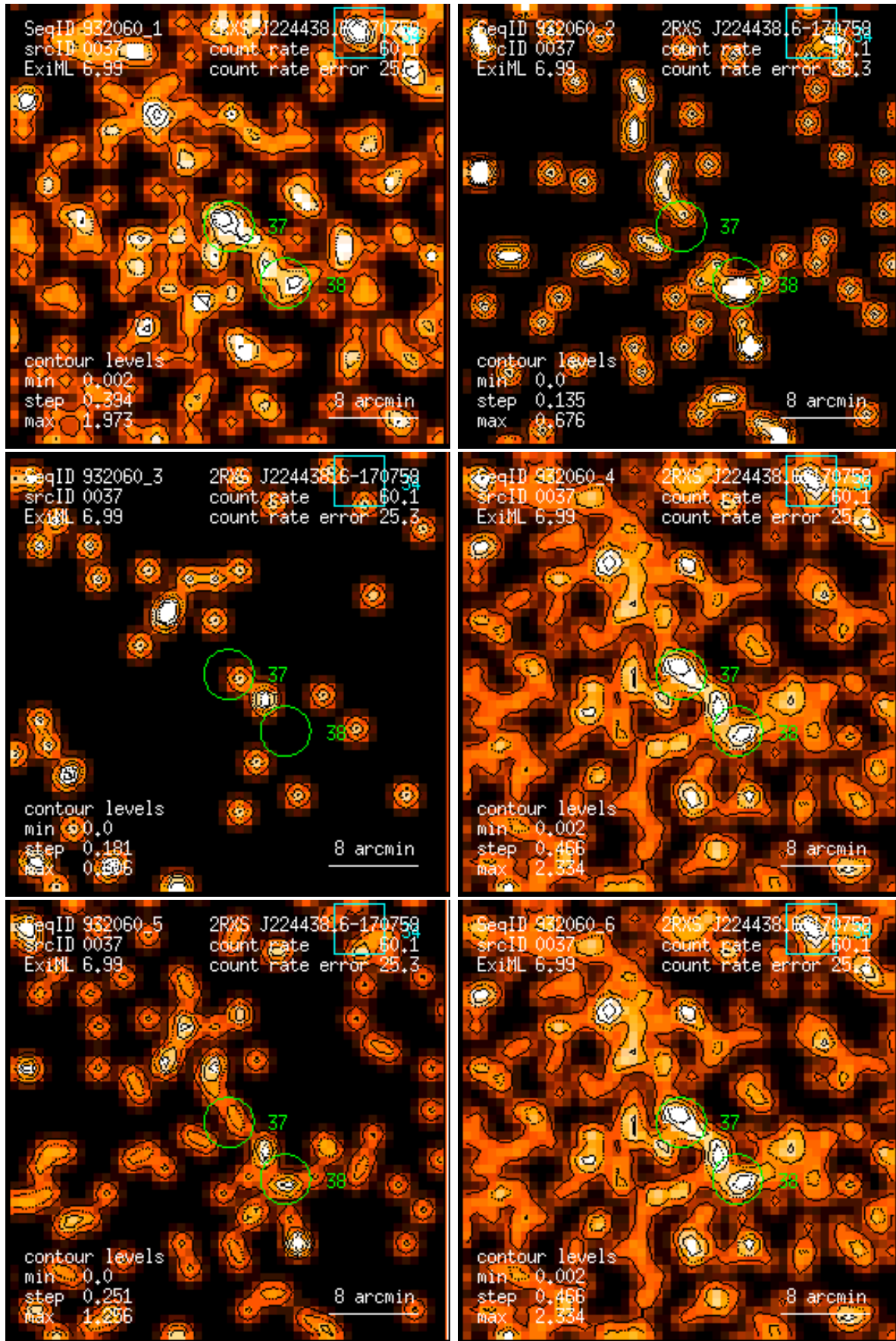
Figure 37: RASS 932060: detection 0037: band rate images, Gaussian filter: (1) PSPC channels 11 – 41, (2) 52 – 90, (3) 91 – 201, (4) 11 – 235, (5) 52 – 201, (6) 11 – 201. Broad band rates in counts/ks. Band rate contour levels in counts/ks/arcmin 2 .
