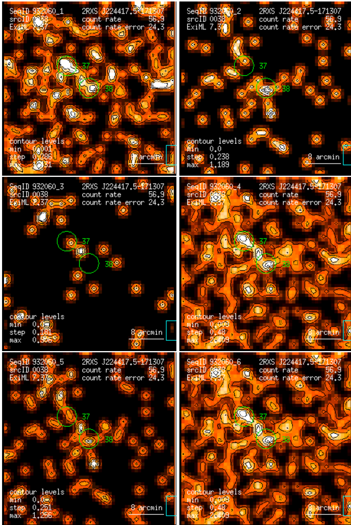
Figure 38: RASS 932060: detection 0038: band rate images, Gaussian filter: (1) PSPC channels 11 – 41, (2) 52 – 90, (3) 91 – 201, (4) 11 – 235, (5) 52 – 201, (6) 11 – 201. Broad band rates in counts/ks. Band rate contour levels in counts/ks/arcmin 2 .
