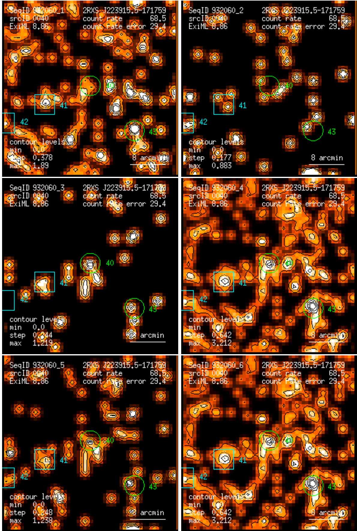
Figure 40: RASS 932060: detection 0040: band rate images, Gaussian filter: (1) PSPC channels 11 – 41, (2) 52 – 90, (3) 91 – 201, (4) 11 – 235, (5) 52 – 201, (6) 11 – 201. Broad band rates in counts/ks. Band rate contour levels in counts/ks/arcmin 2 .
