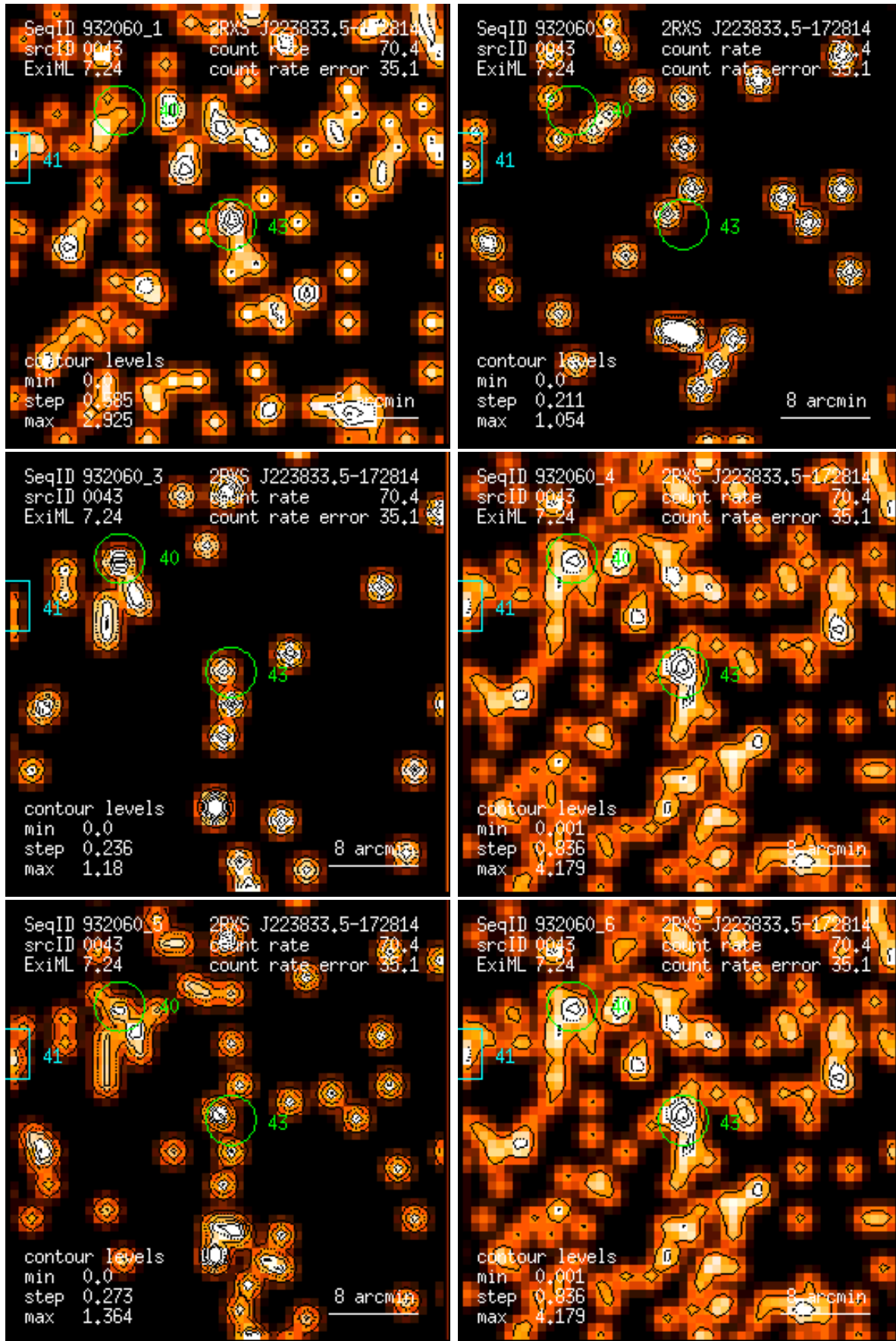
Figure 43: RASS 932060: detection 0043: band rate images, Gaussian filter: (1) PSPC channels 11 – 41, (2) 52 – 90, (3) 91 – 201, (4) 11 – 235, (5) 52 – 201, (6) 11 – 201. Broad band rates in counts/ks. Band rate contour levels in counts/ks/arcmin 2 .
