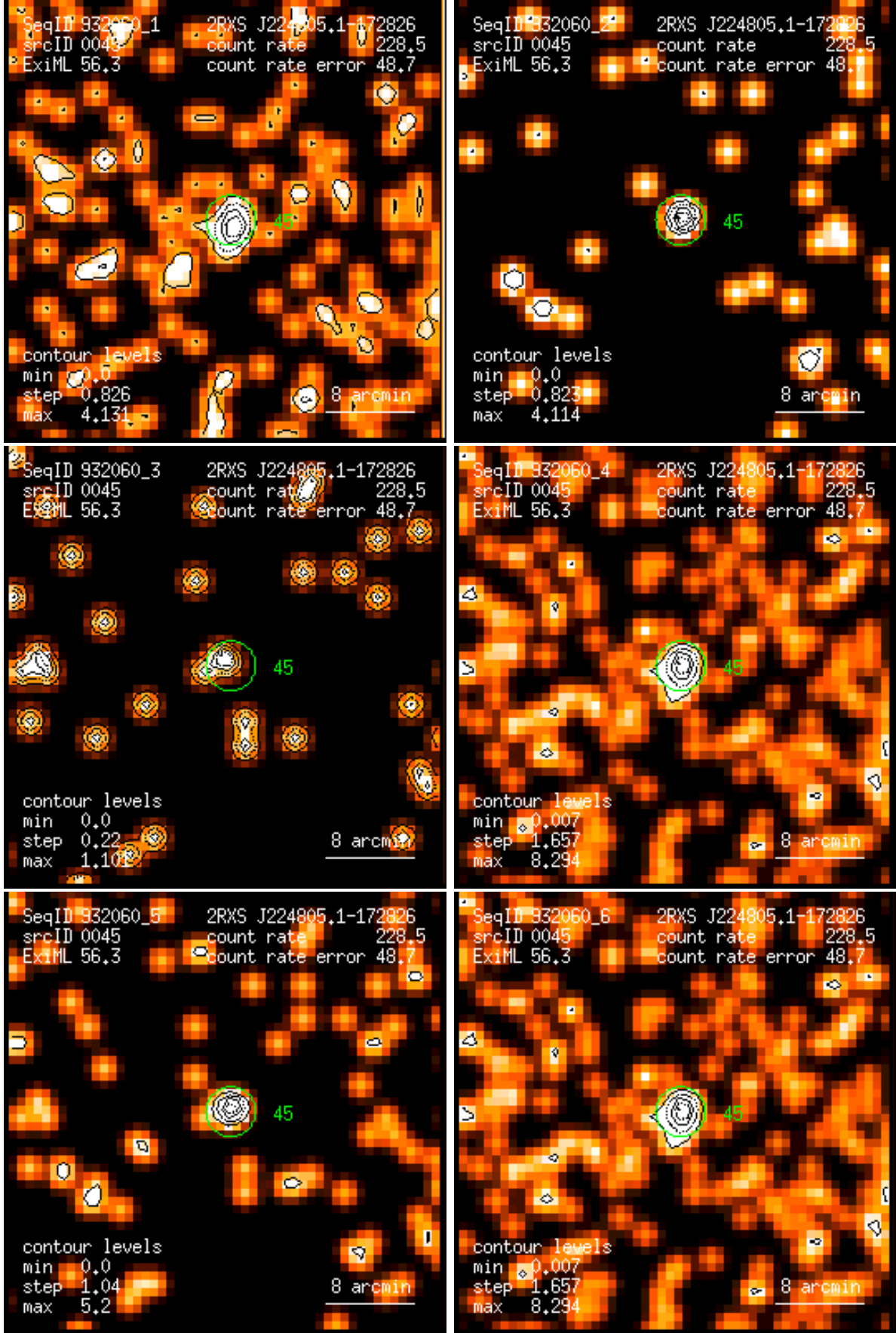
Figure 45: RASS 932060: detection 0045: band rate images, Gaussian filter: (1) PSPC channels 11 – 41, (2) 52 – 90, (3) 91 – 201, (4) 11 – 235, (5) 52 – 201, (6) 11 – 201. Broad band rates in counts/ks. Band rate contour levels in counts/ks/arcmin 2 .
