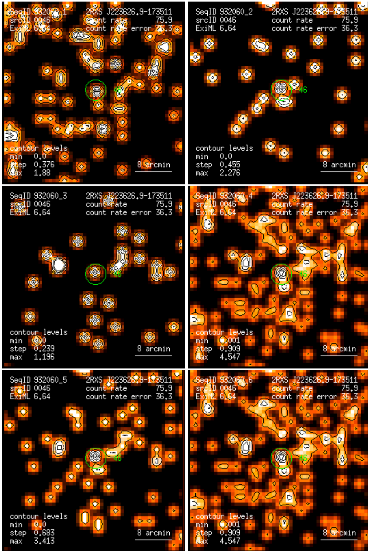
Figure 46: RASS 932060: detection 0046: band rate images, Gaussian filter: (1) PSPC channels 11 – 41, (2) 52 – 90, (3) 91 – 201, (4) 11 – 235, (5) 52 – 201, (6) 11 – 201. Broad band rates in counts/ks. Band rate contour levels in counts/ks/arcmin 2 .
