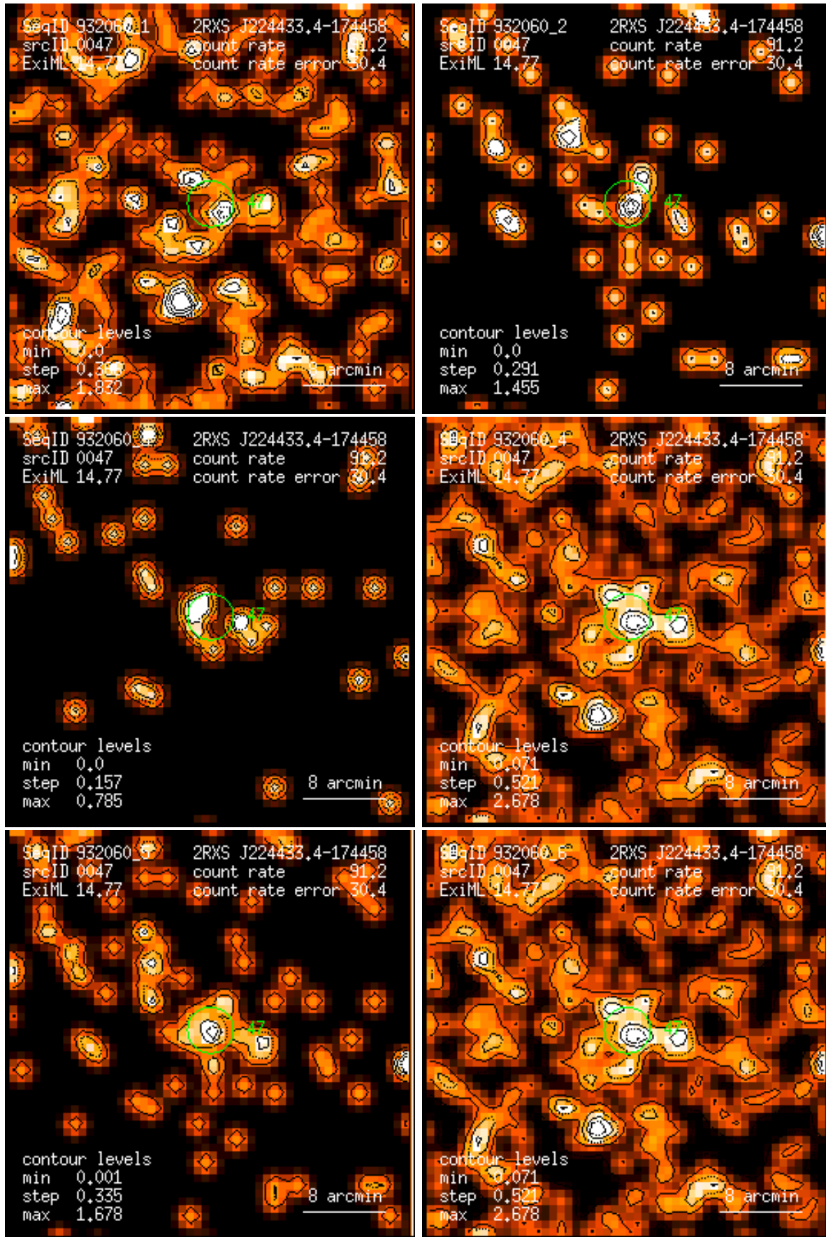
Figure 47: RASS 932060: detection 0047: band rate images, Gaussian filter: (1) PSPC channels 11 – 41, (2) 52 – 90, (3) 91 – 201, (4) 11 – 235, (5) 52 – 201, (6) 11 – 201. Broad band rates in counts/ks. Band rate contour levels in counts/ks/arcmin 2 .
