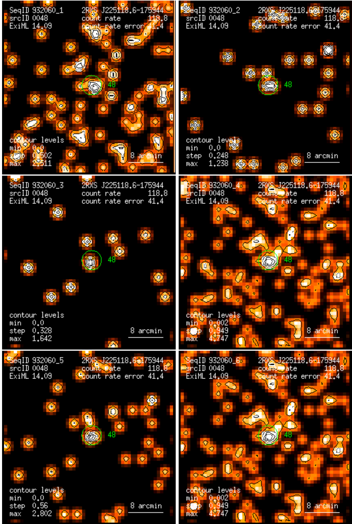
Figure 48: RASS 932060: detection 0048: band rate images, Gaussian filter: (1) PSPC channels 11 – 41, (2) 52 – 90, (3) 91 – 201, (4) 11 – 235, (5) 52 – 201, (6) 11 – 201. Broad band rates in counts/ks. Band rate contour levels in counts/ks/arcmin 2 .
