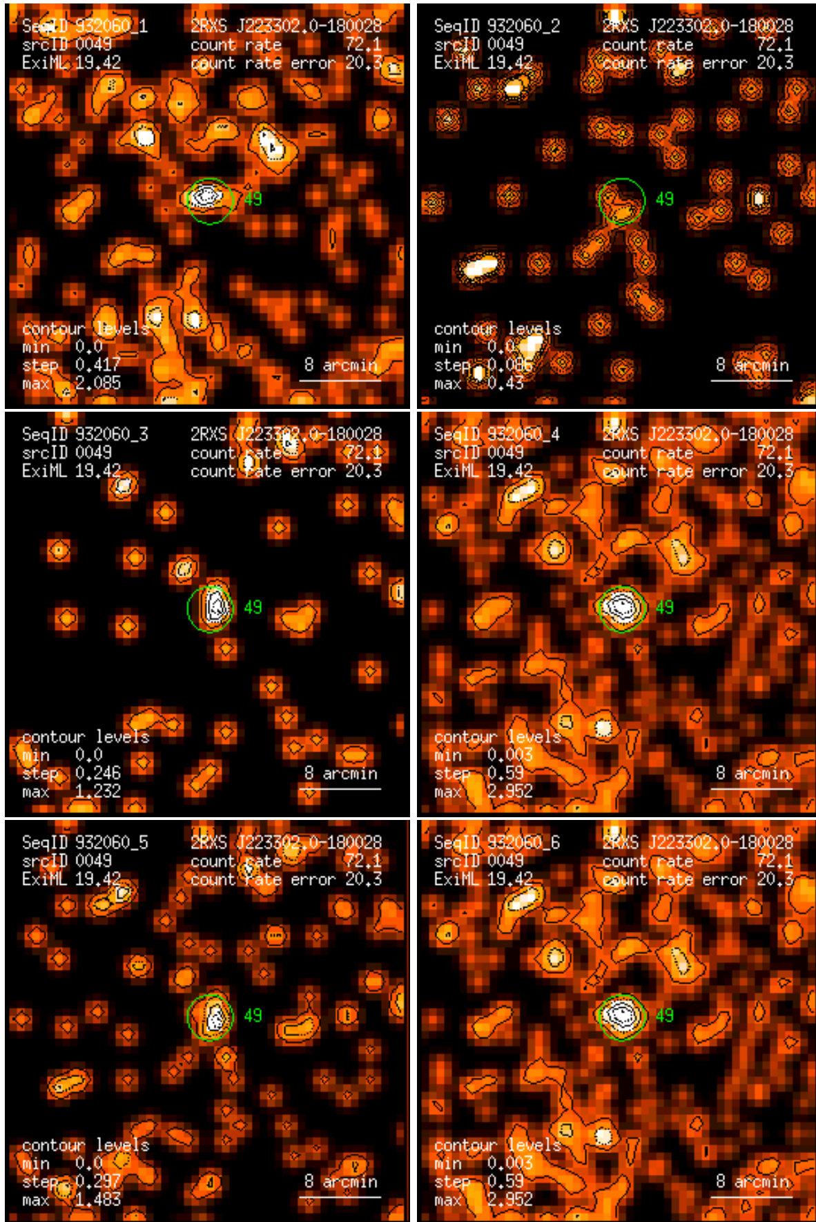
Figure 49: RASS 932060: detection 0049: band rate images, Gaussian filter: (1) PSPC channels 11 – 41, (2) 52 – 90, (3) 91 – 201, (4) 11 – 235, (5) 52 – 201, (6) 11 – 201. Broad band rates in counts/ks. Band rate contour levels in counts/ks/arcmin 2 .
