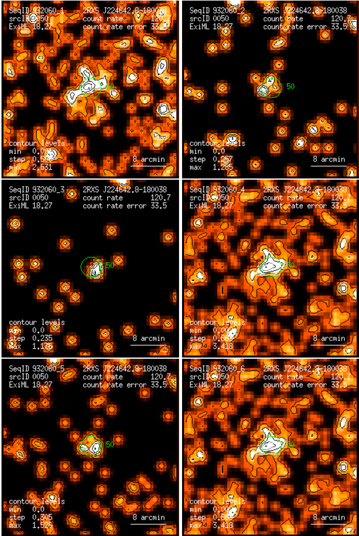
Figure 50: RASS 932060: detection 0050: band rate images, Gaussian filter: (1) PSPC channels 11 – 41, (2) 52 – 90, (3) 91 – 201, (4) 11 – 235, (5) 52 – 201, (6) 11 – 201. Broad band rates in counts/ks. Band rate contour levels in counts/ks/arcmin 2 .
