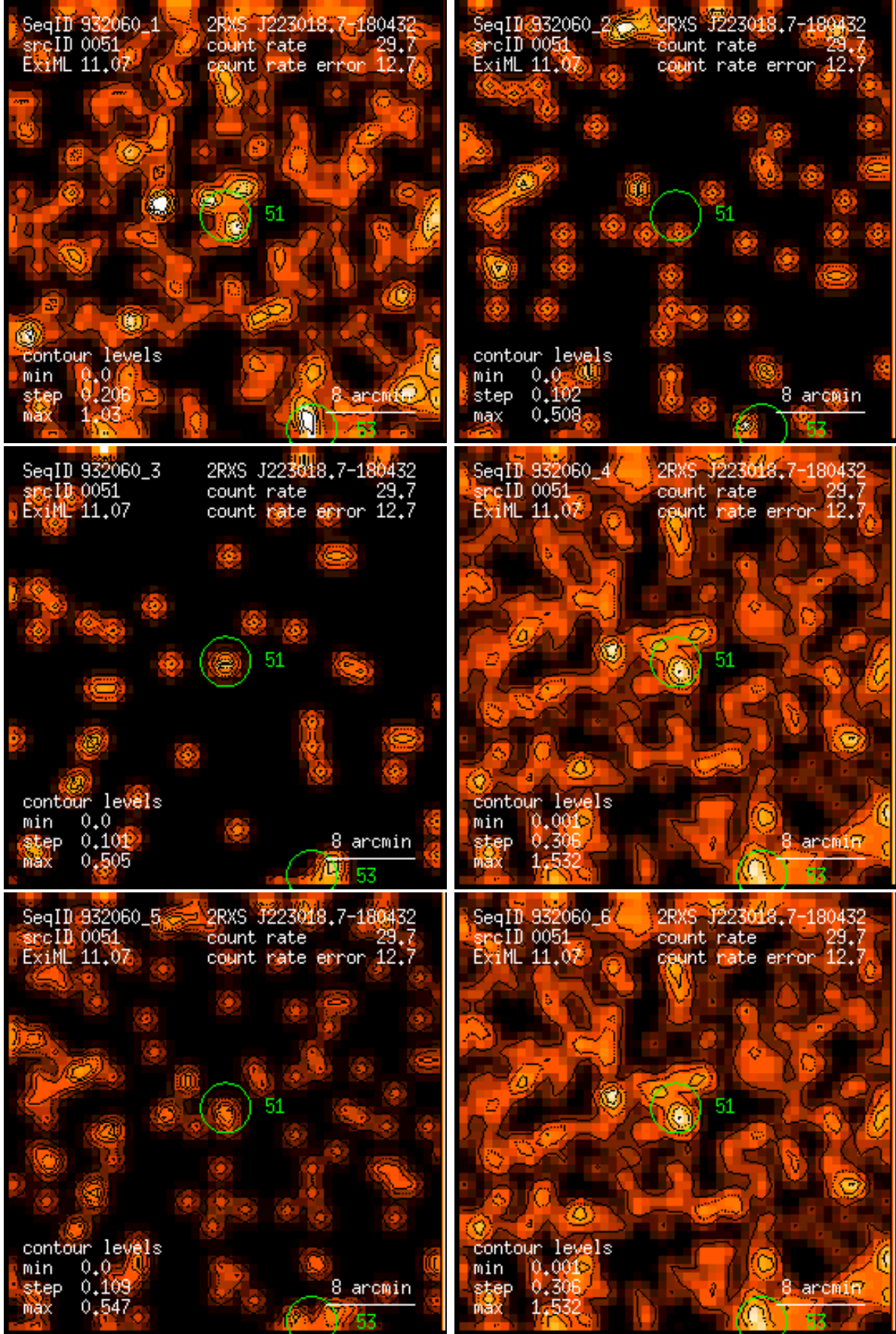
Figure 51: RASS 932060: detection 0051: band rate images, Gaussian filter: (1) PSPC channels 11 – 41, (2) 52 – 90, (3) 91 – 201, (4) 11 – 235, (5) 52 – 201, (6) 11 – 201. Broad band rates in counts/ks. Band rate contour levels in counts/ks/arcmin 2 .
