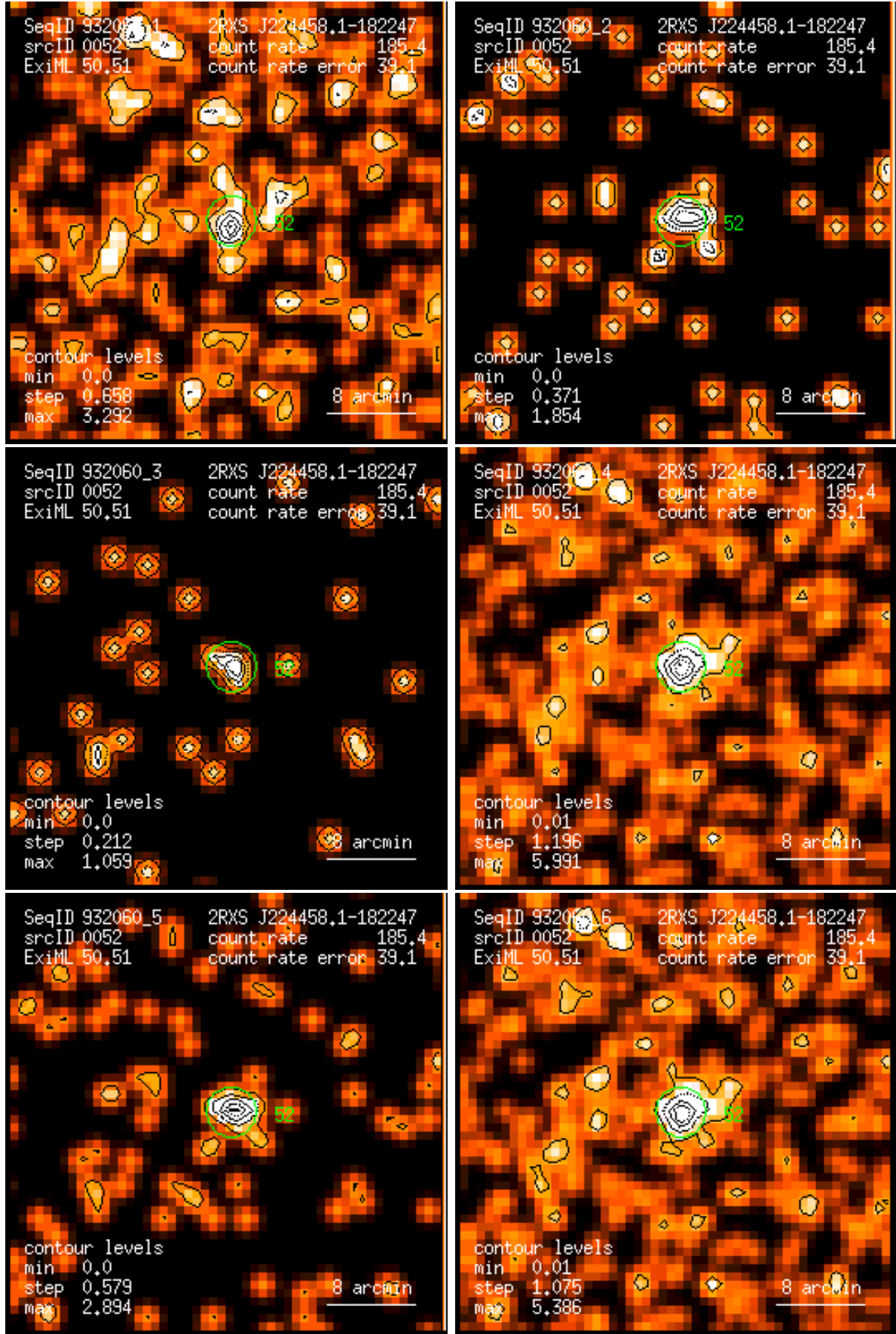
Figure 52: RASS 932060: detection 0052: band rate images, Gaussian filter: (1) PSPC channels 11 – 41, (2) 52 – 90, (3) 91 – 201, (4) 11 – 235, (5) 52 – 201, (6) 11 – 201. Broad band rates in counts/ks. Band rate contour levels in counts/ks/arcmin 2 .
