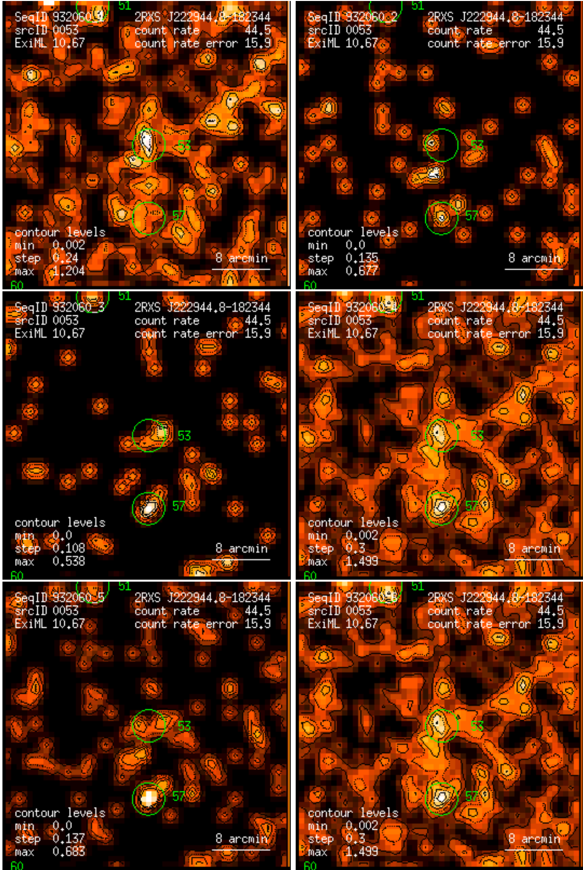
Figure 53: RASS 932060: detection 0053: band rate images, Gaussian filter: (1) PSPC channels 11 – 41, (2) 52 – 90, (3) 91 – 201, (4) 11 – 235, (5) 52 – 201, (6) 11 – 201. Broad band rates in counts/ks. Band rate contour levels in counts/ks/arcmin 2 .
