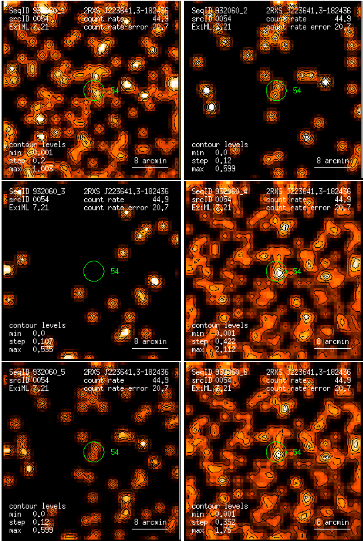
Figure 54: RASS 932060: detection 0054: band rate images, Gaussian filter: (1) PSPC channels 11 – 41, (2) 52 – 90, (3) 91 – 201, (4) 11 – 235, (5) 52 – 201, (6) 11 – 201. Broad band rates in counts/ks. Band rate contour levels in counts/ks/arcmin 2 .
