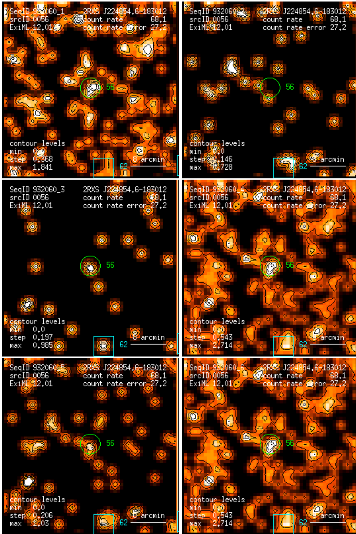
Figure 56: RASS 932060: detection 0056: band rate images, Gaussian filter: (1) PSPC channels 11 – 41, (2) 52 – 90, (3) 91 – 201, (4) 11 – 235, (5) 52 – 201, (6) 11 – 201. Broad band rates in counts/ks. Band rate contour levels in counts/ks/arcmin 2 .
