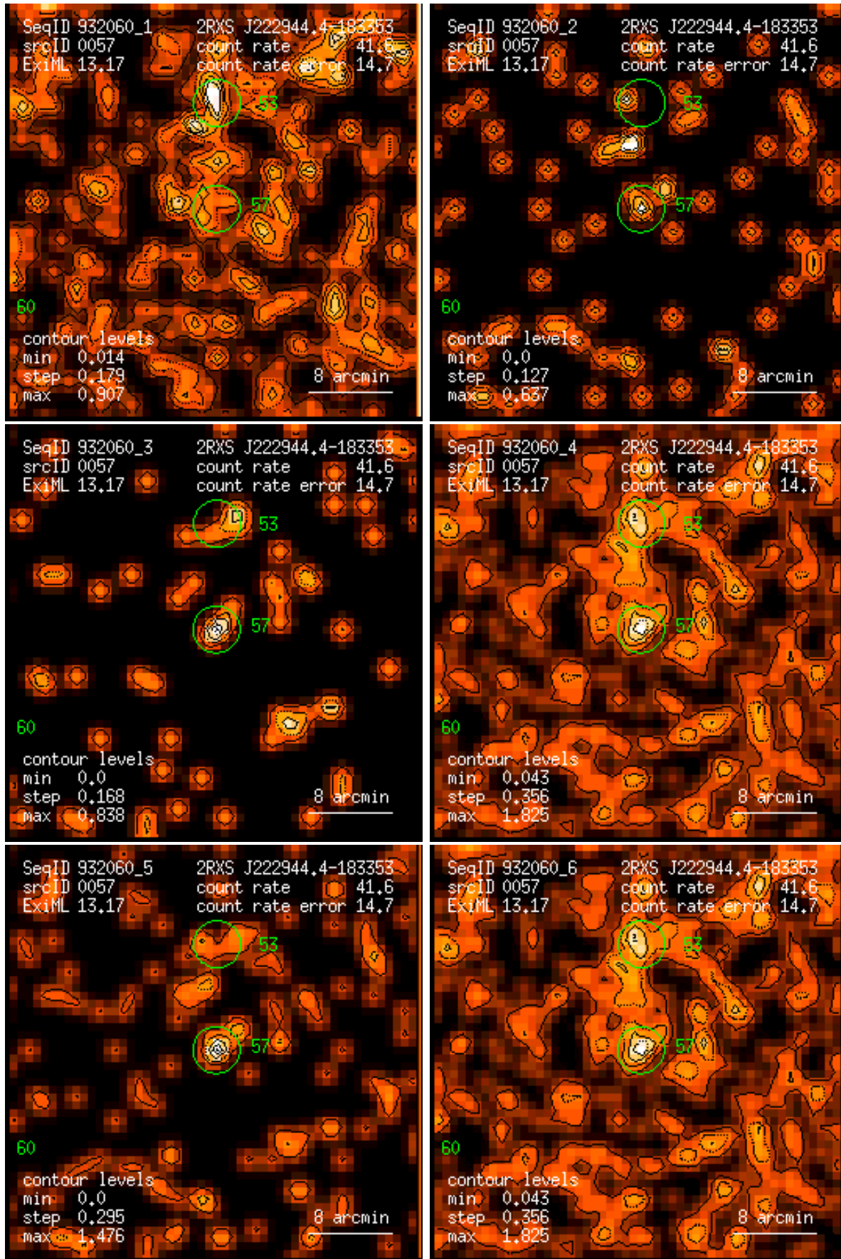
Figure 57: RASS 932060: detection 0057: band rate images, Gaussian filter: (1) PSPC channels 11 – 41, (2) 52 – 90, (3) 91 – 201, (4) 11 – 235, (5) 52 – 201, (6) 11 – 201. Broad band rates in counts/ks. Band rate contour levels in counts/ks/arcmin 2 .
