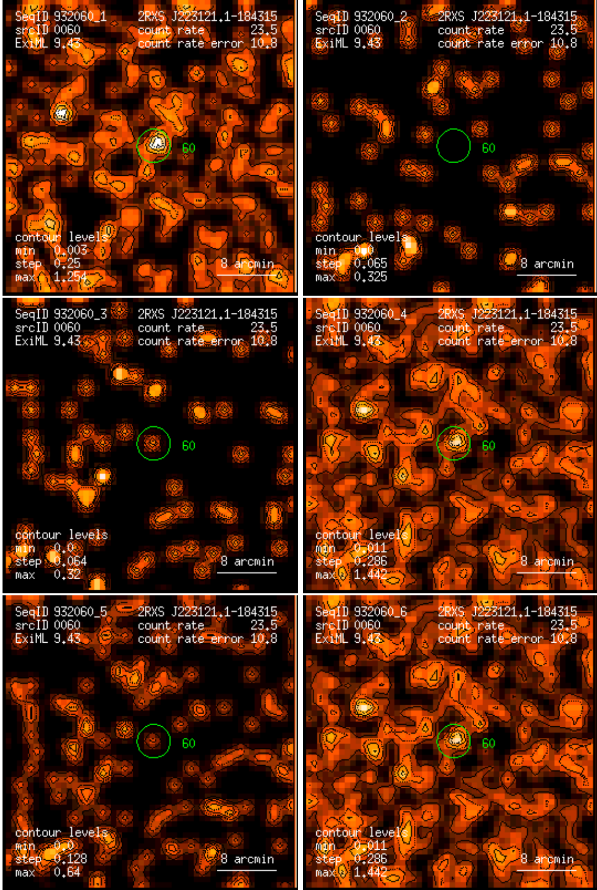
Figure 60: RASS 932060: detection 0060: band rate images, Gaussian filter: (1) PSPC channels 11 – 41, (2) 52 – 90, (3) 91 – 201, (4) 11 – 235, (5) 52 – 201, (6) 11 – 201. Broad band rates in counts/ks. Band rate contour levels in counts/ks/arcmin 2 .
