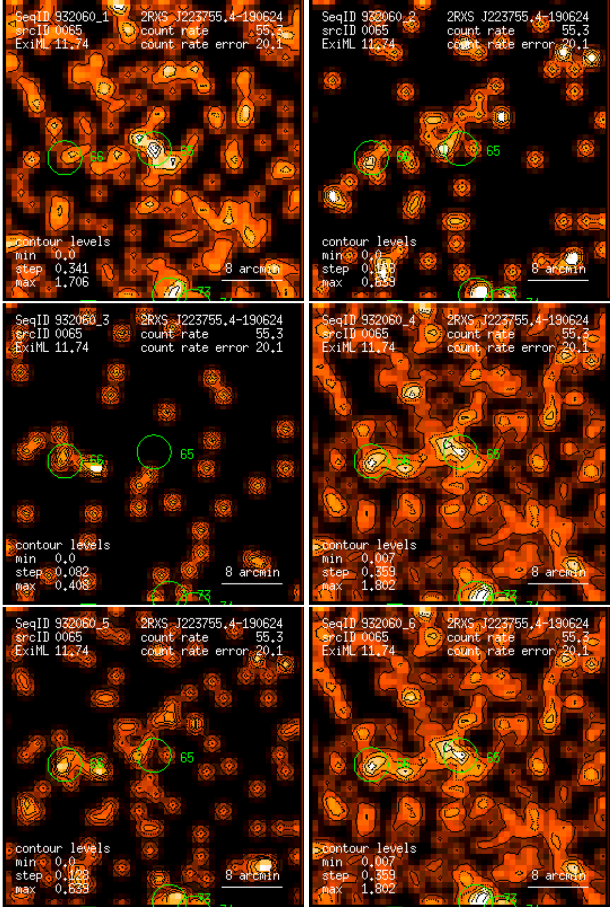
Figure 65: RASS 932060: detection 0065: band rate images, Gaussian filter: (1) PSPC channels 11 – 41, (2) 52 – 90, (3) 91 – 201, (4) 11 – 235, (5) 52 – 201, (6) 11 – 201. Broad band rates in counts/ks. Band rate contour levels in counts/ks/arcmin 2 .
