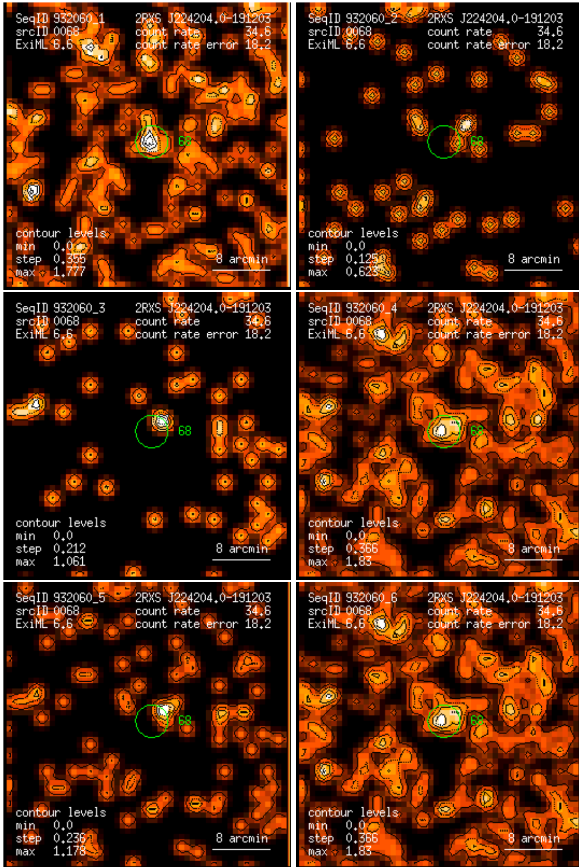
Figure 68: RASS 932060: detection 0068: band rate images, Gaussian filter: (1) PSPC channels 11 – 41, (2) 52 – 90, (3) 91 – 201, (4) 11 – 235, (5) 52 – 201, (6) 11 – 201. Broad band rates in counts/ks. Band rate contour levels in counts/ks/arcmin 2 .
