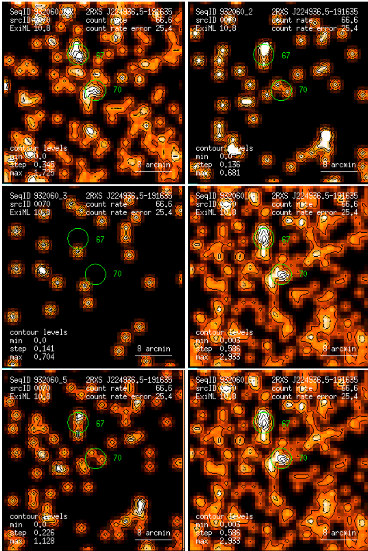
Figure 70: RASS 932060: detection 0070: band rate images, Gaussian filter: (1) PSPC channels 11 – 41, (2) 52 – 90, (3) 91 – 201, (4) 11 – 235, (5) 52 – 201, (6) 11 – 201. Broad band rates in counts/ks. Band rate contour levels in counts/ks/arcmin 2 .
