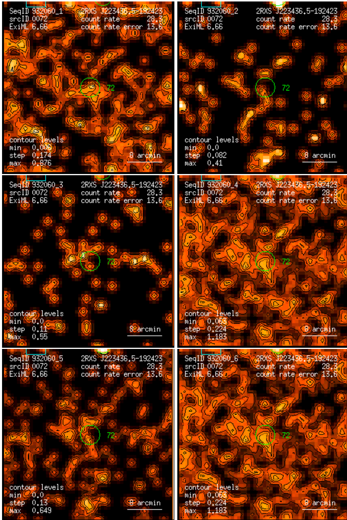
Figure 72: RASS 932060: detection 0072: band rate images, Gaussian filter: (1) PSPC channels 11 – 41, (2) 52 – 90, (3) 91 – 201, (4) 11 – 235, (5) 52 – 201, (6) 11 – 201. Broad band rates in counts/ks. Band rate contour levels in counts/ks/arcmin 2 .
