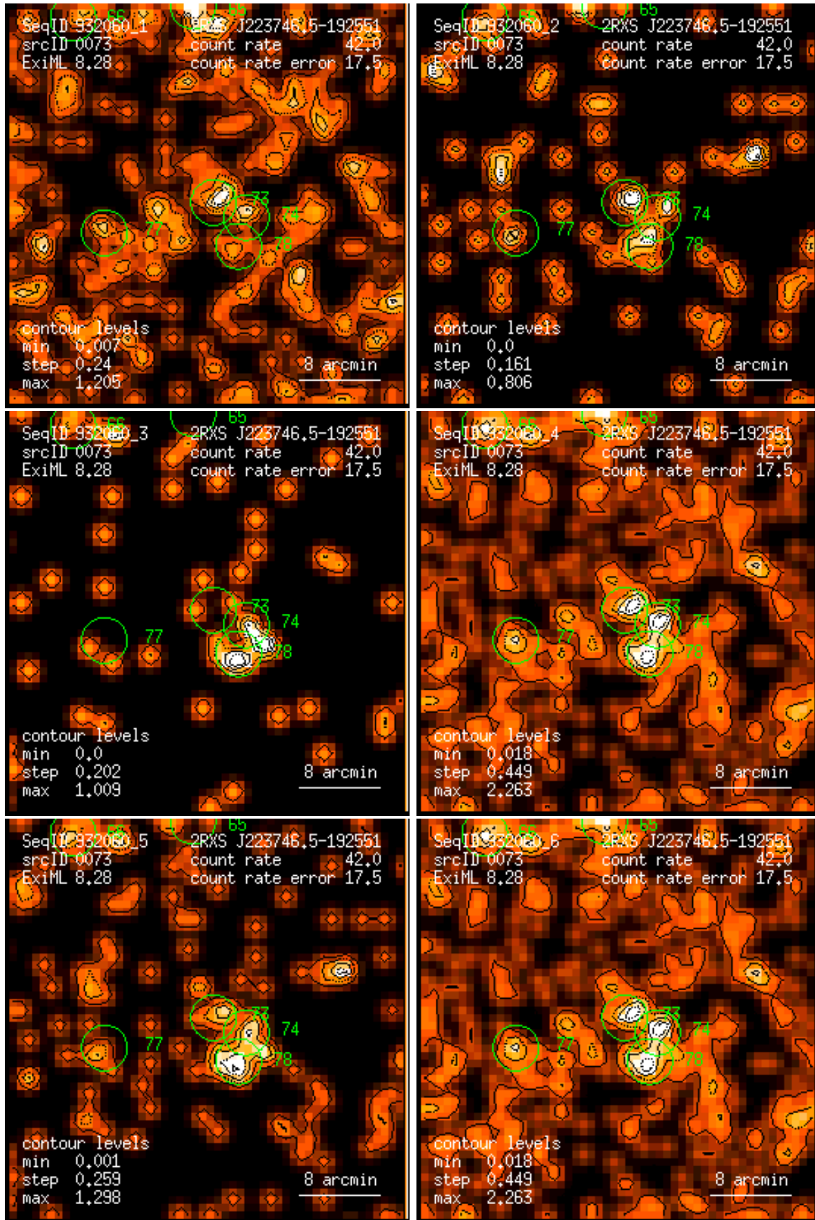
Figure 73: RASS 932060: detection 0073: band rate images, Gaussian filter: (1) PSPC channels 11 – 41, (2) 52 – 90, (3) 91 – 201, (4) 11 – 235, (5) 52 – 201, (6) 11 – 201. Broad band rates in counts/ks. Band rate contour levels in counts/ks/arcmin 2 .
