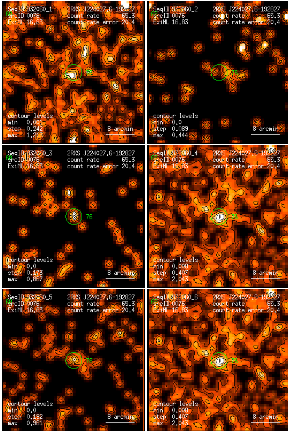
Figure 76: RASS 932060: detection 0076: band rate images, Gaussian filter: (1) PSPC channels 11 – 41, (2) 52 – 90, (3) 91 – 201, (4) 11 – 235, (5) 52 – 201, (6) 11 – 201. Broad band rates in counts/ks. Band rate contour levels in counts/ks/arcmin 2 .
