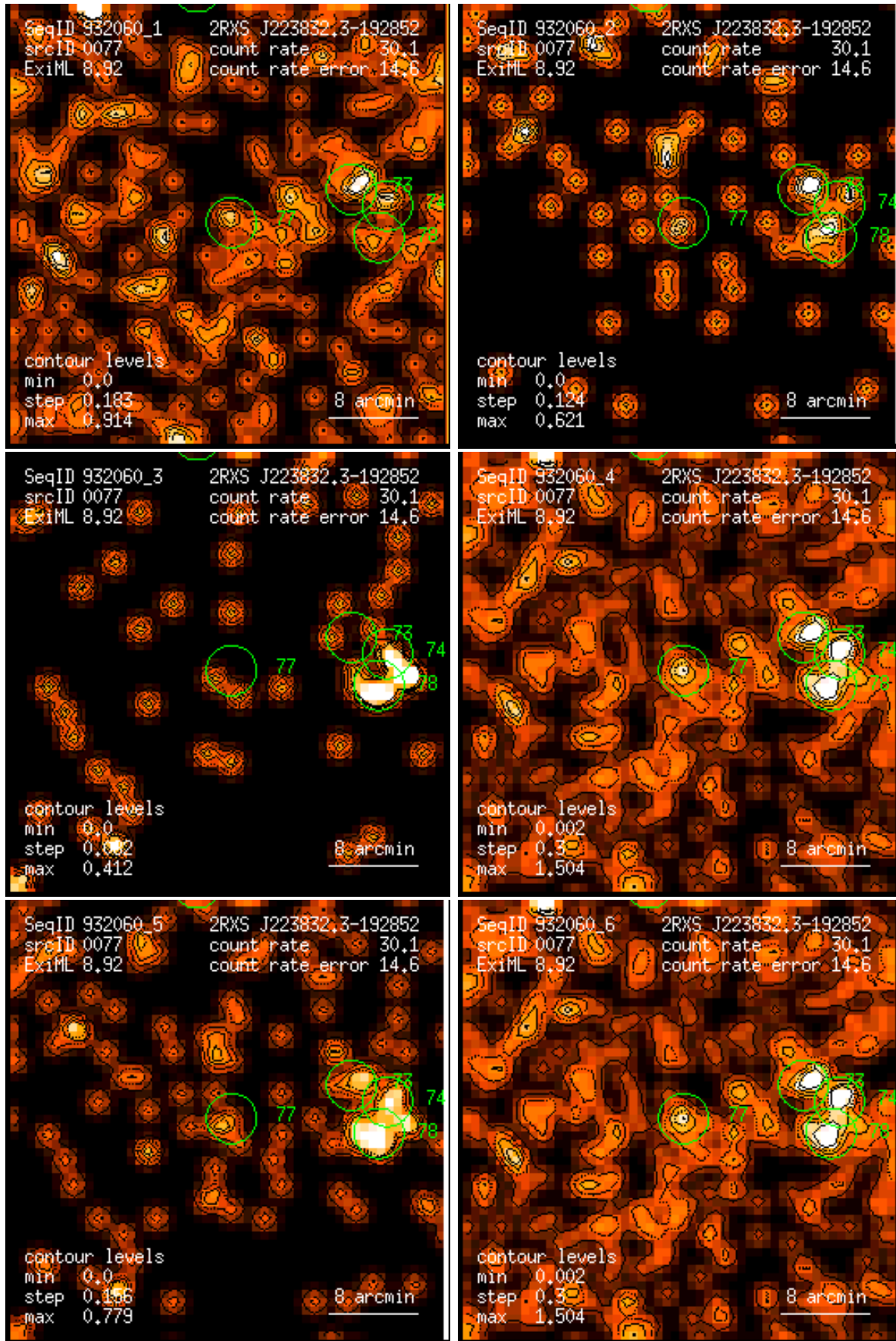
Figure 77: RASS 932060: detection 0077: band rate images, Gaussian filter: (1) PSPC channels 11 – 41, (2) 52 – 90, (3) 91 – 201, (4) 11 – 235, (5) 52 – 201, (6) 11 – 201. Broad band rates in counts/ks. Band rate contour levels in counts/ks/arcmin 2 .
