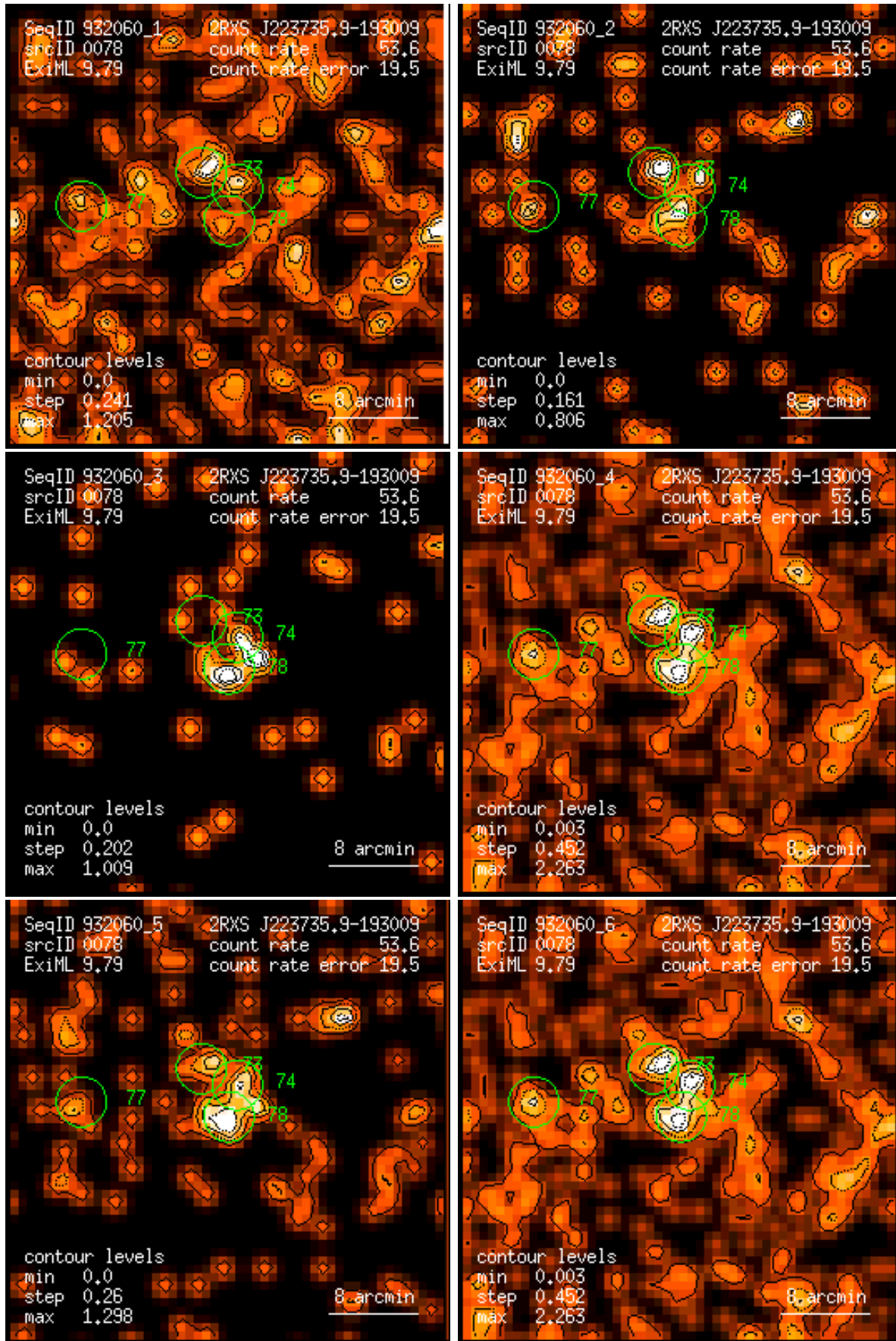
Figure 78: RASS 932060: detection 0078: band rate images, Gaussian filter: (1) PSPC channels 11 – 41, (2) 52 – 90, (3) 91 – 201, (4) 11 – 235, (5) 52 – 201, (6) 11 – 201. Broad band rates in counts/ks. Band rate contour levels in counts/ks/arcmin 2 .
