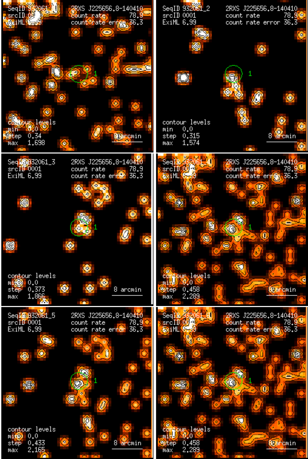
Figure 1: RASS 932061: detection 0001: band rate images, Gaussian filter: (1) PSPC channels 11 – 41, (2) 52 – 90, (3) 91 – 201, (4) 11 – 235, (5) 52 – 201, (6) 11 – 201. Broad band rates in counts/ks. Band rate contour levels in counts/ks/arcmin 2 .
