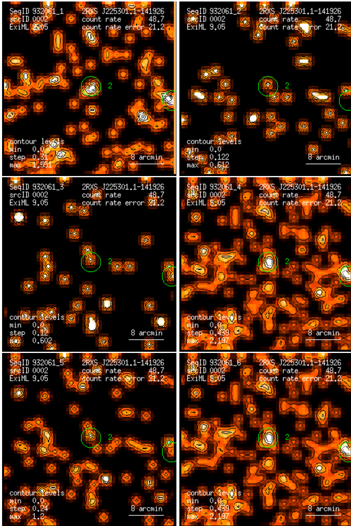
Figure 2: RASS 932061: detection 0002: band rate images, Gaussian filter: (1) PSPC channels 11 – 41, (2) 52 – 90, (3) 91 – 201, (4) 11 – 235, (5) 52 – 201, (6) 11 – 201. Broad band rates in counts/ks. Band rate contour levels in counts/ks/arcmin 2 .
