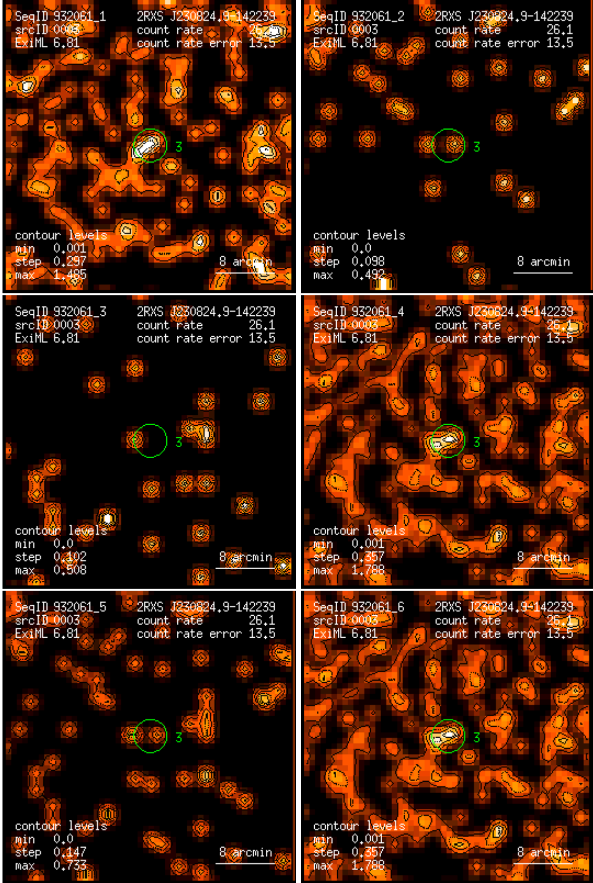
Figure 3: RASS 932061: detection 0003: band rate images, Gaussian filter: (1) PSPC channels 11 – 41, (2) 52 – 90, (3) 91 – 201, (4) 11 – 235, (5) 52 – 201, (6) 11 – 201. Broad band rates in counts/ks. Band rate contour levels in counts/ks/arcmin 2 .
