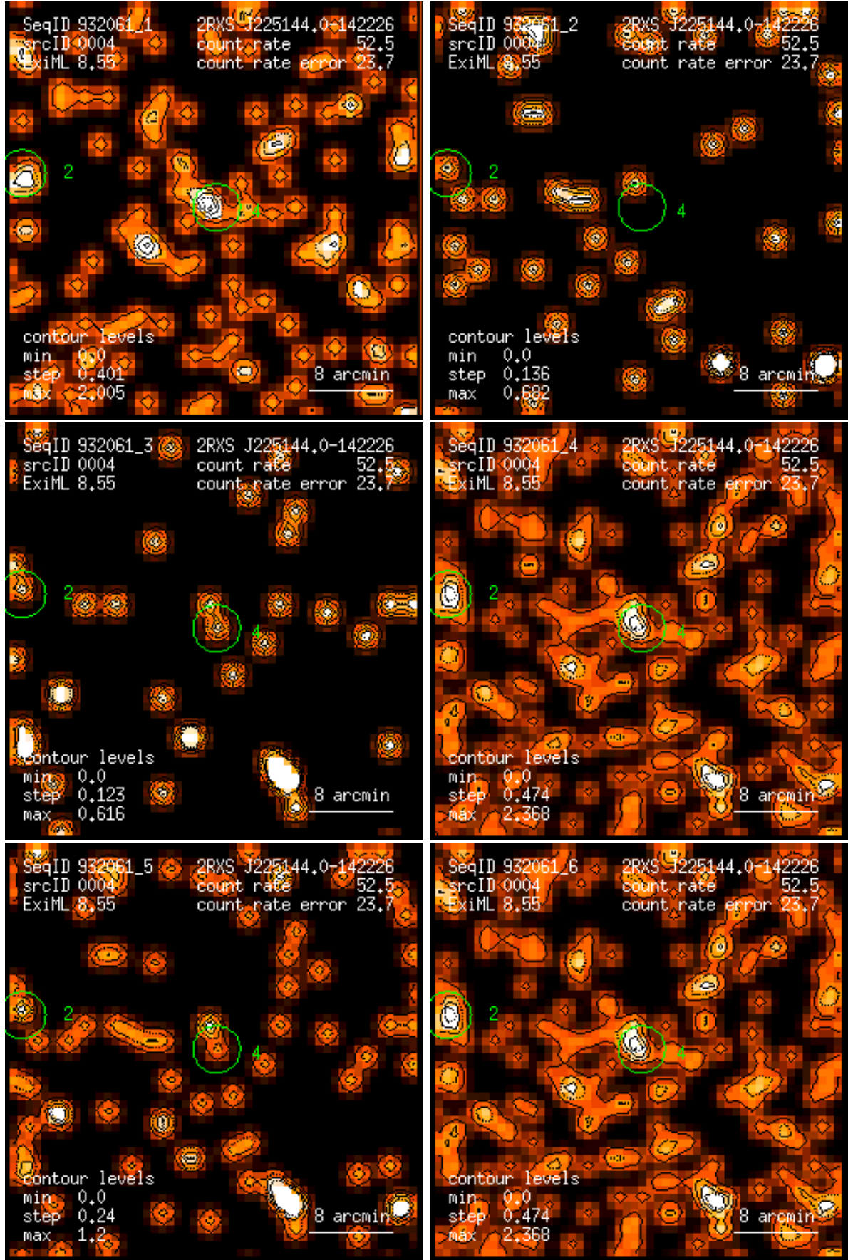
Figure 4: RASS 932061: detection 0004: band rate images, Gaussian filter: (1) PSPC channels 11 – 41, (2) 52 – 90, (3) 91 – 201, (4) 11 – 235, (5) 52 – 201, (6) 11 – 201. Broad band rates in counts/ks. Band rate contour levels in counts/ks/arcmin 2 .
